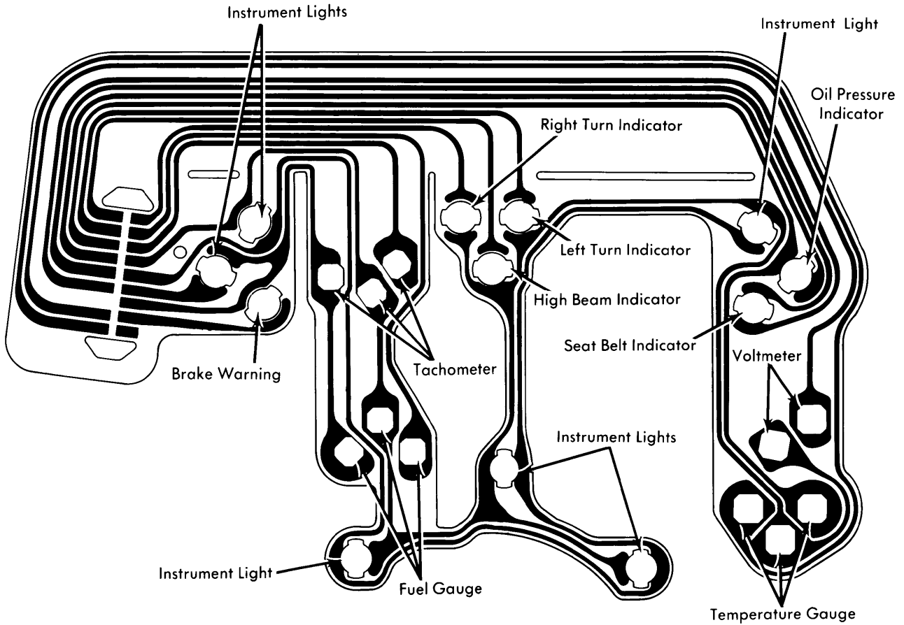
Monza and Town Coupe Instrument Cluster with Gauges
