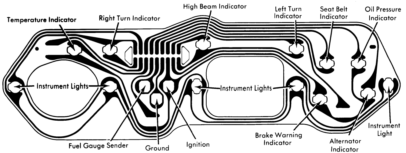
Nova Instrument Cluster with Indicator Lights
