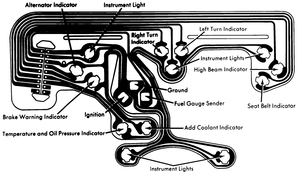
Monza and Town Coupe Instrument Cluster with Indicator Lights
