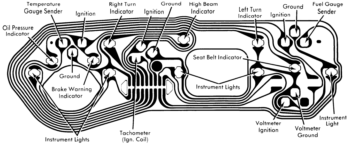
Nova Instrument Cluster with Gauges
