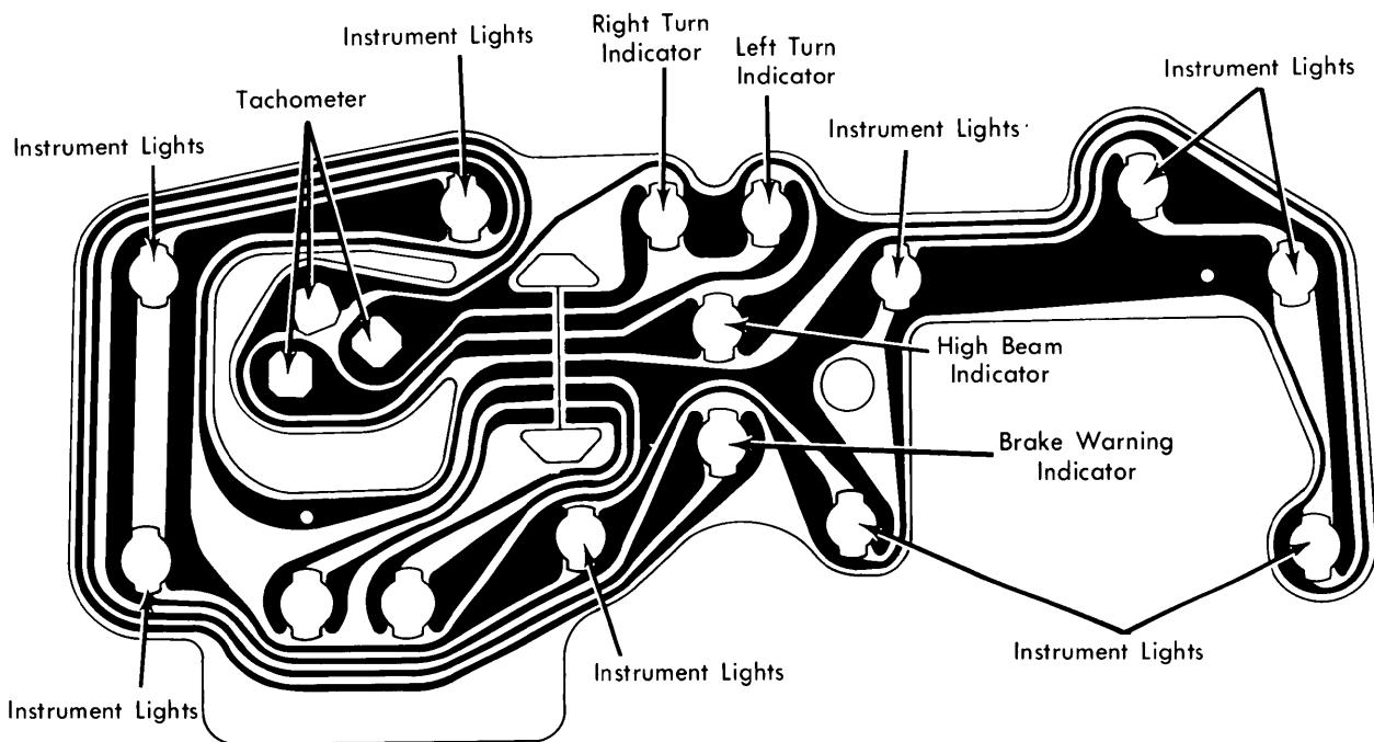
Corvette Instrument Panel Gauge Cluster
