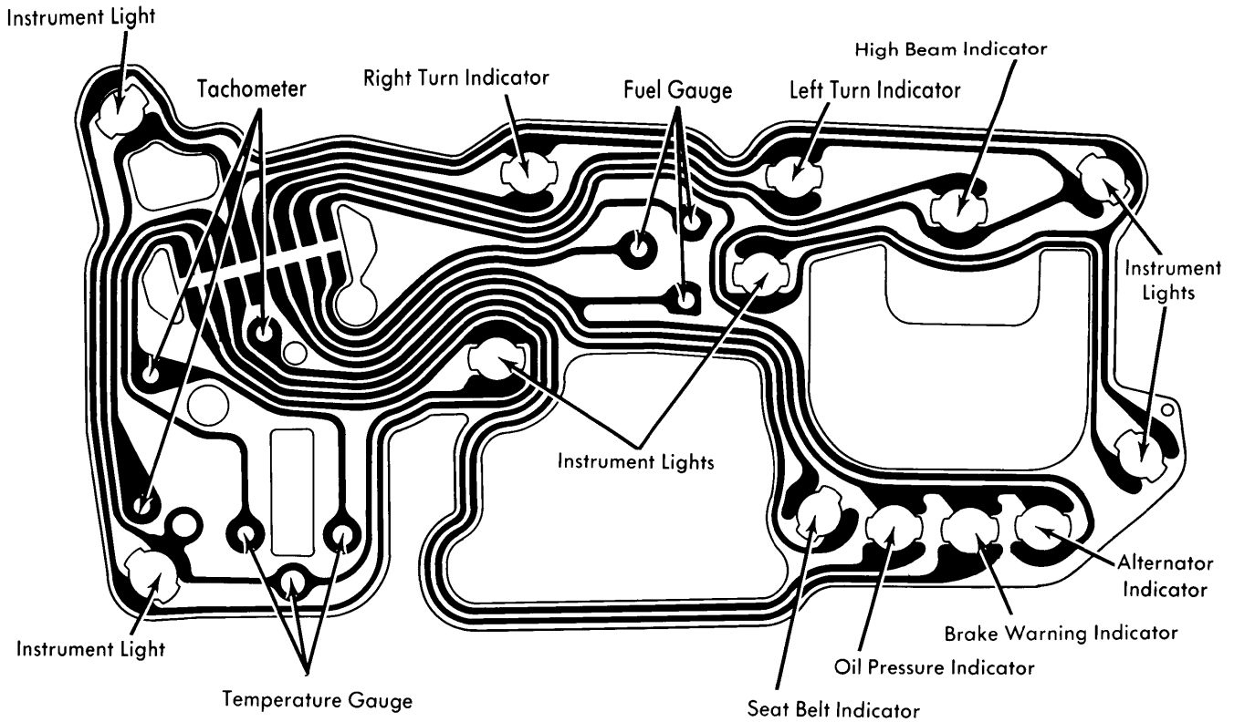
Chevette Instrument Cluster with Gauges
