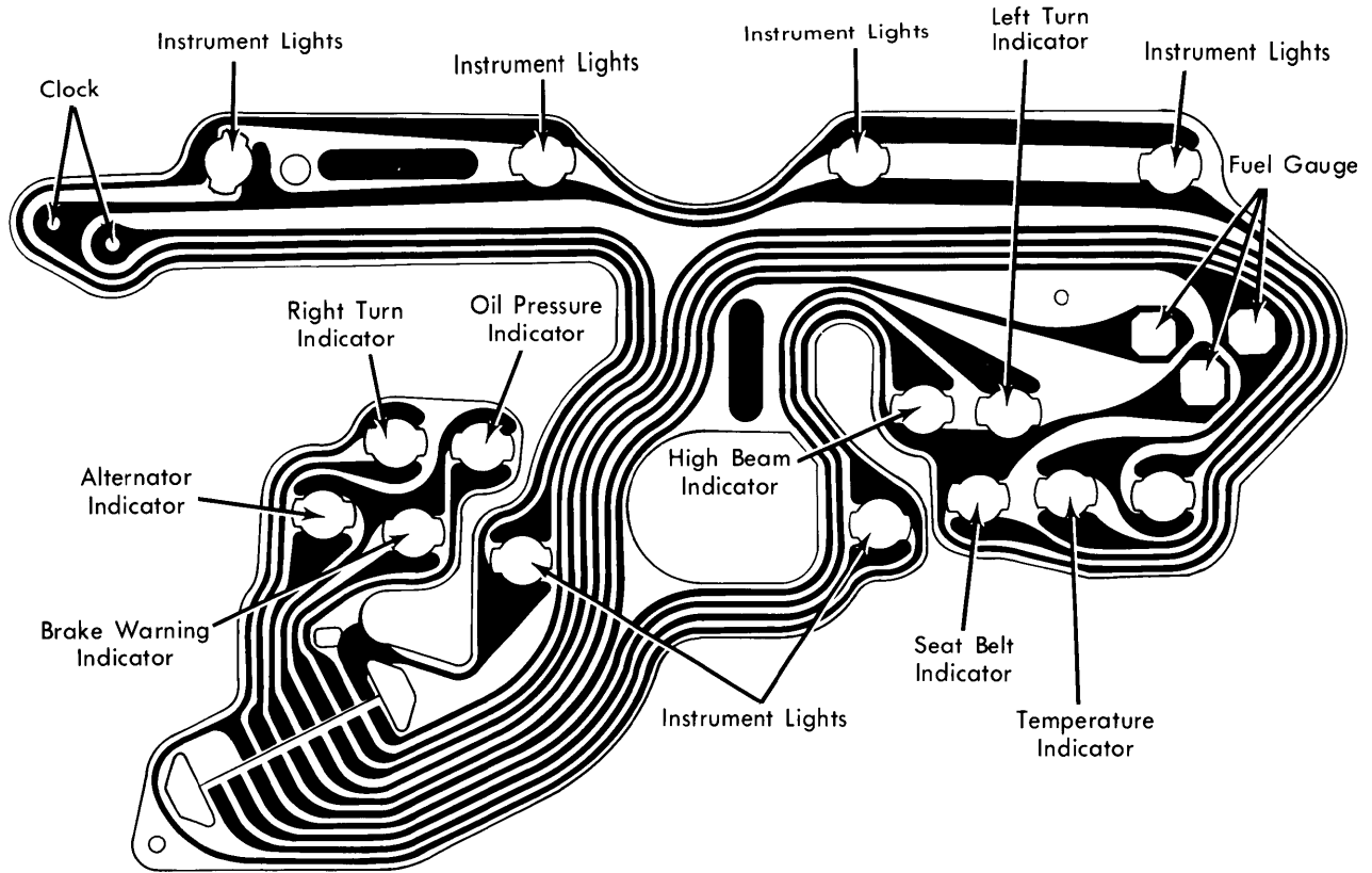
Malibu, Monte Carlo & El Camino Instrument Cluster without Gauges
