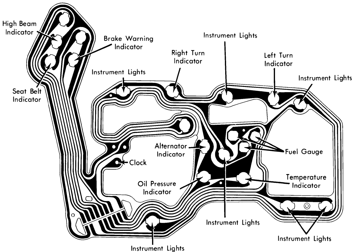
Malibu, Monte Carlo & El Camino Instrument Cluster without Gauges
