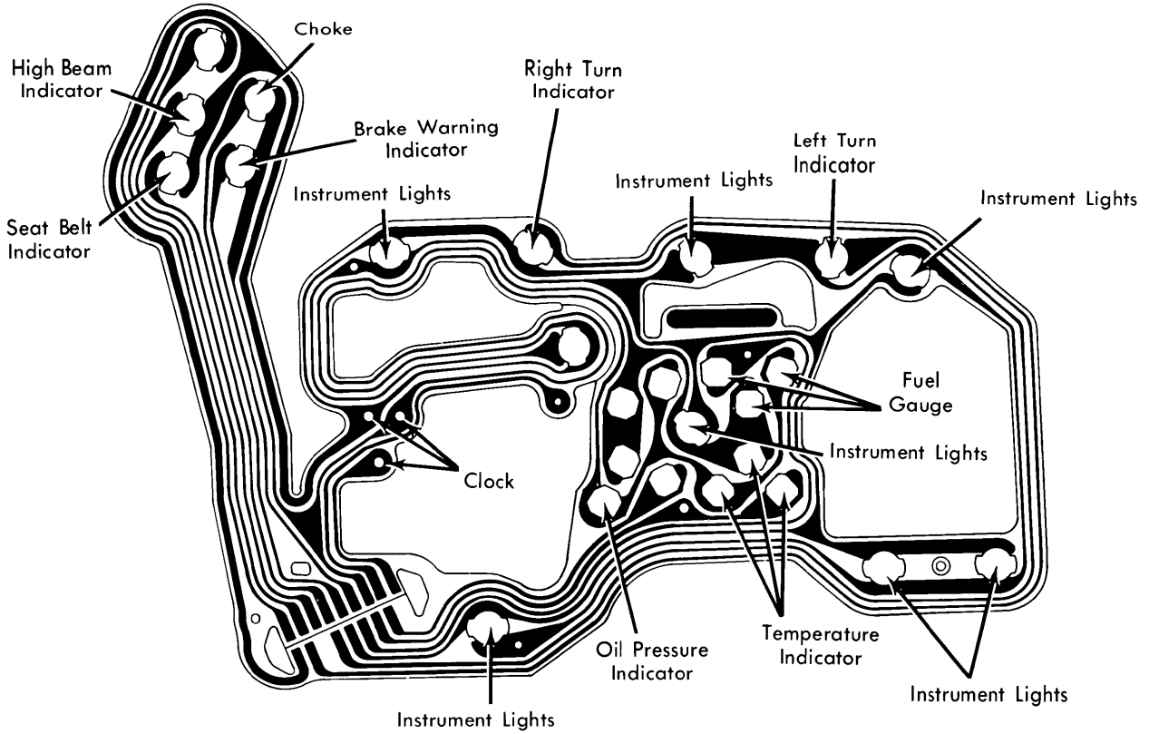
Malibu, Monte Carlo & El Camino Instrument Cluster with Gauges
