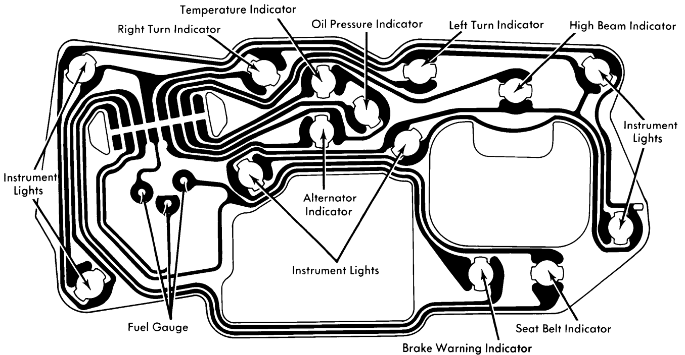
Chevette Instrument Cluster with Indicator Lights
