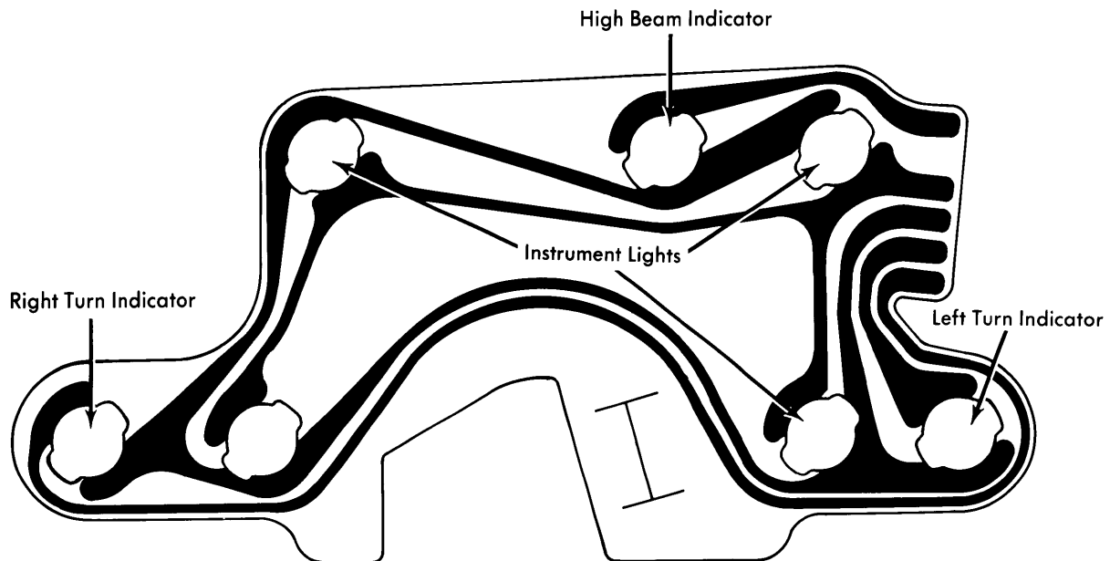
Cadillac (except Seville and Eldorado) Speedometer Cluster
