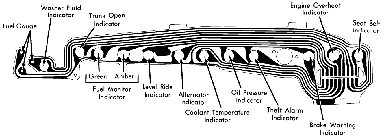
Seville Instrument Cluster without Digital Readout
