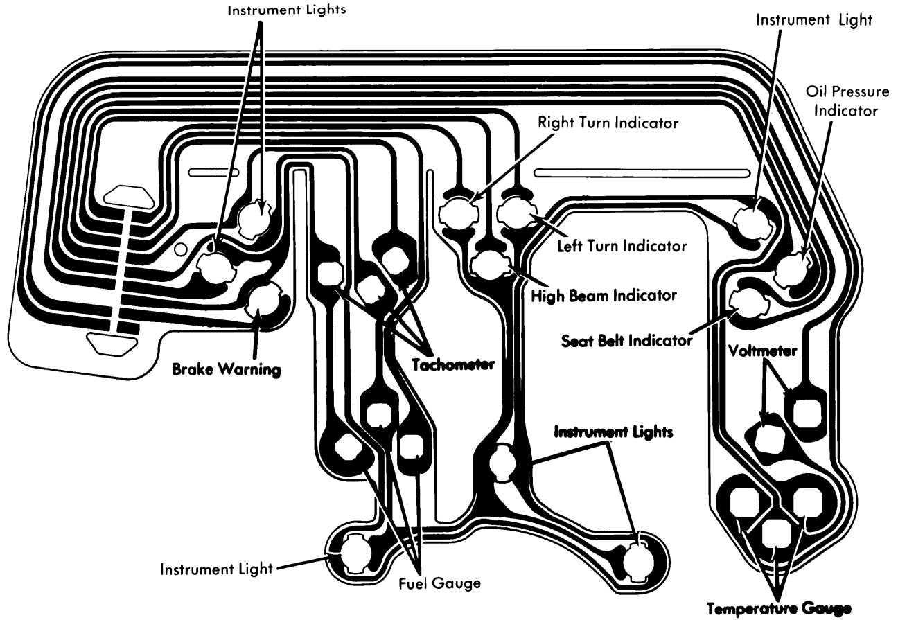
Skyhawk Instrument Cluster with Gauges
