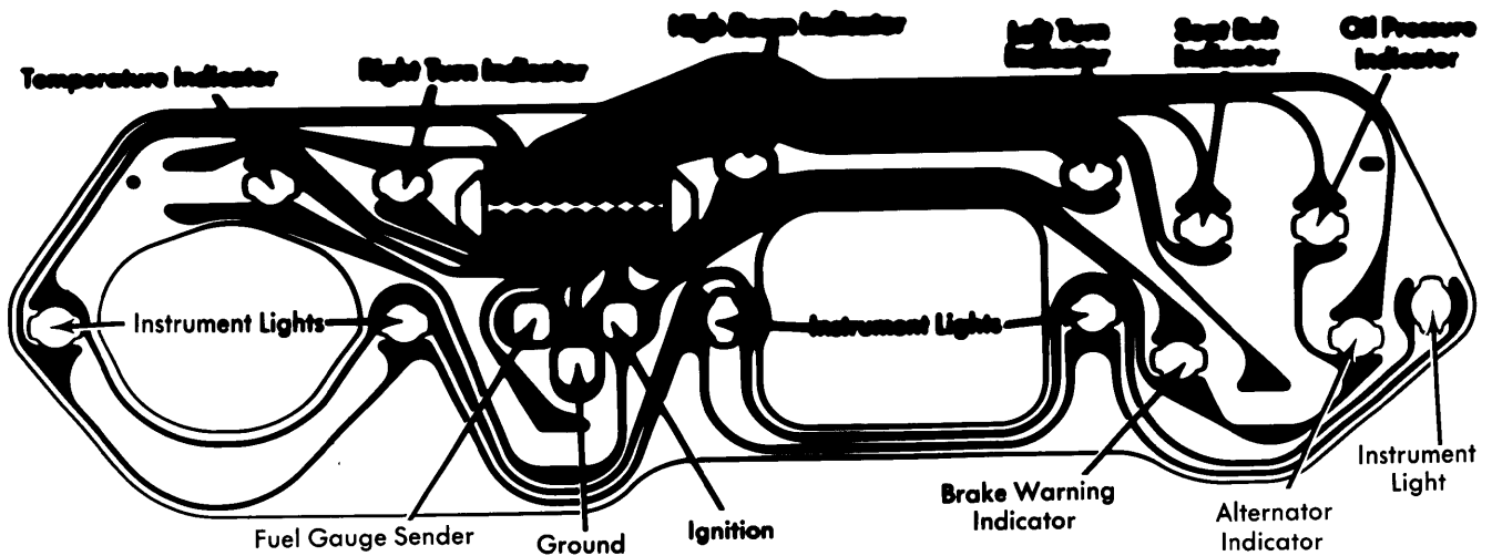
Skylark Instrument Cluster with Indicator Lights
