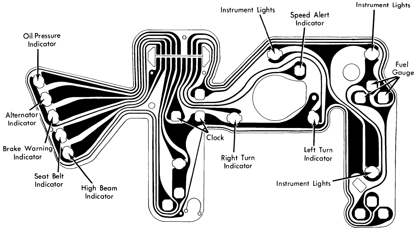
Century & Regal Instrument Cluster with Gauges
