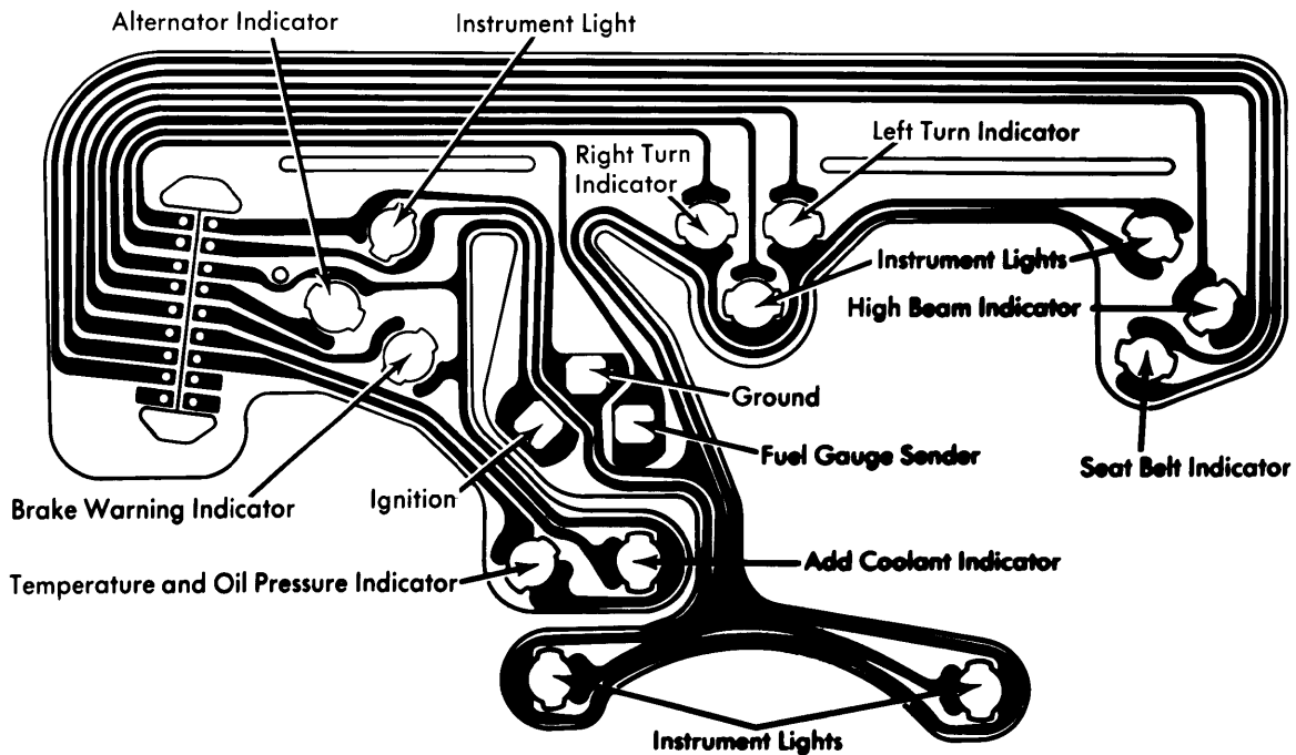
Skyhawk Instrument Cluster with Indicator Lights
