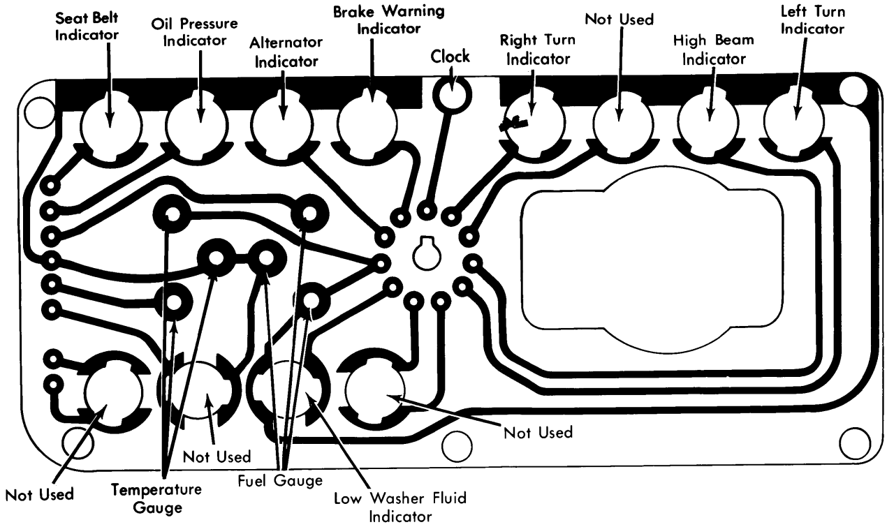
Gremlin, Concord and AMX Instrument Cluster
