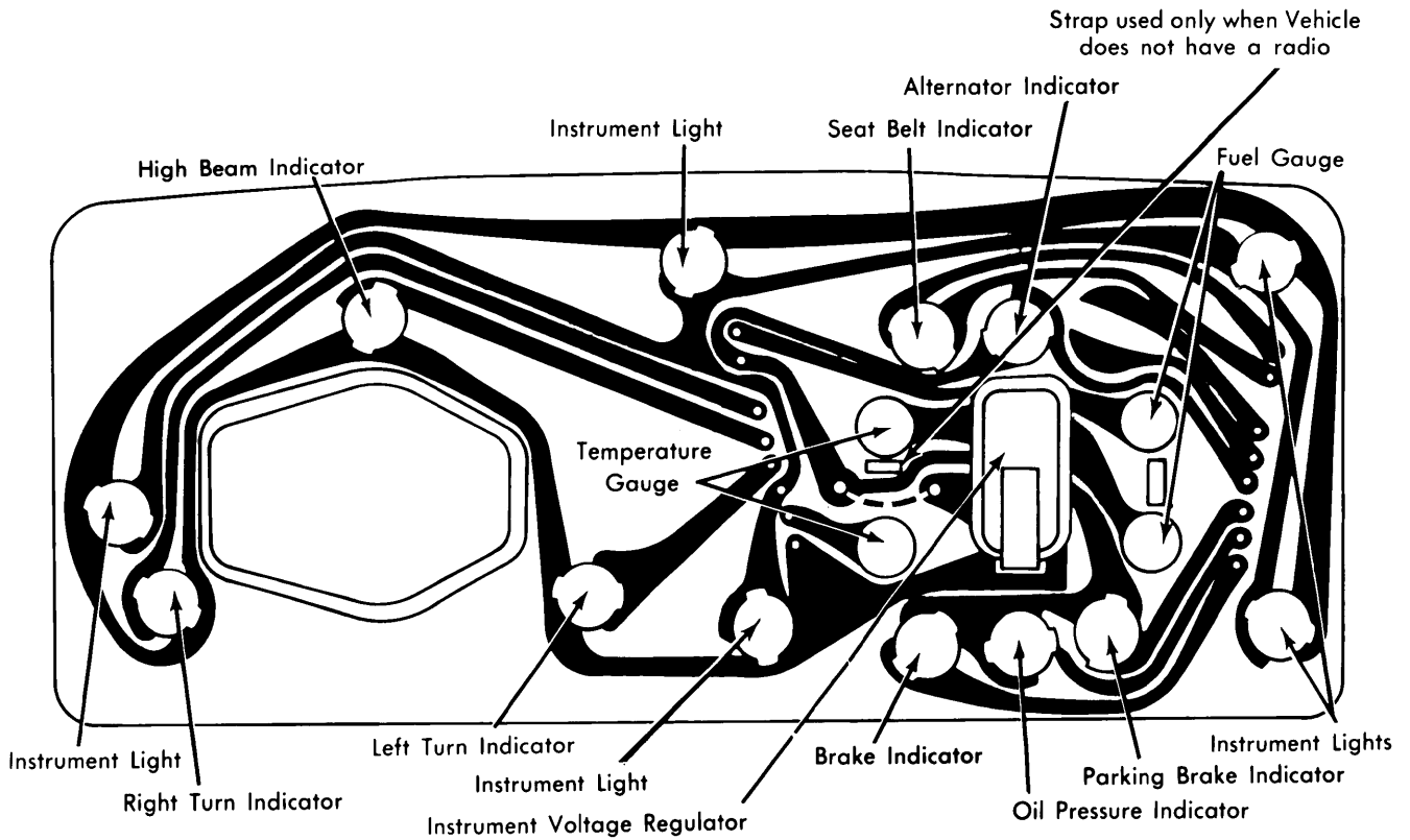
Matador Instrument Cluster with Fuel Economy Gauge in Clock Opening
