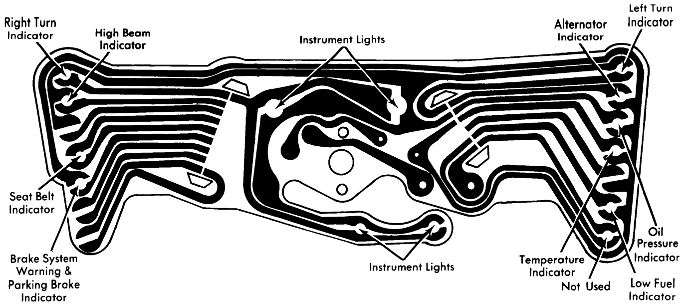
Pacer Instrument Cluster with Indicator Lights
