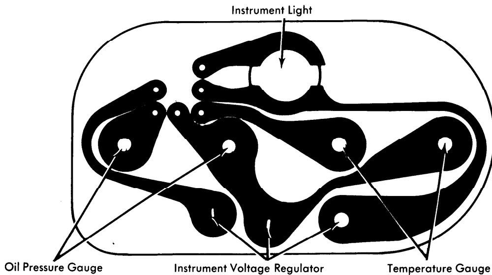
International Harvester Scout II, Traveler and Terra Temperature and Oil Pressure Gauge Circuit
