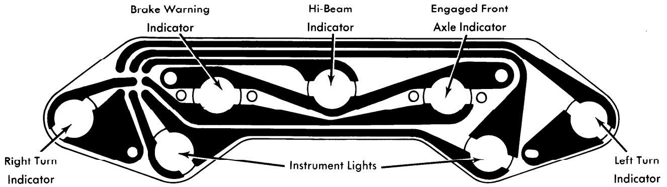
International Harvester Scout II, Traveler and Terra Speedometer Circuit
