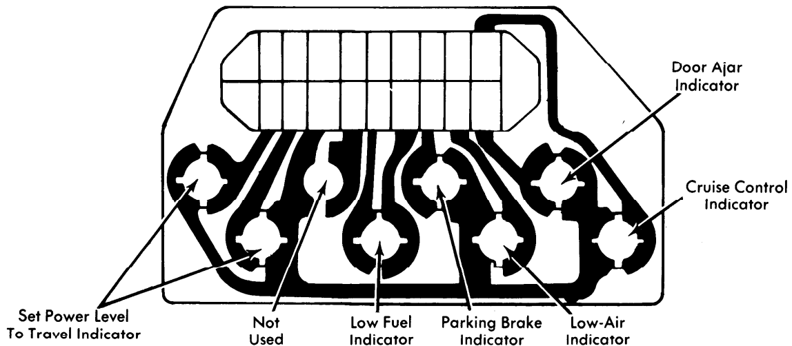
GMC Front Wheel Drive Motor Home Tell-Tale Circuit
