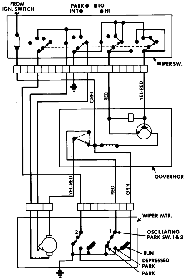
Ford Motor Co. Two-Speed Depressed Park Intermittent Wiper System Wiring Diagram - LTD II, Cougar, Thunderbird, Ford, Mercury, Lincoln and Mark V
