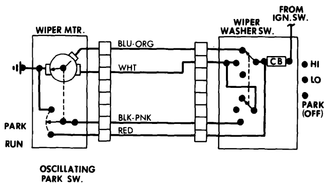
Ford Motor Co. Non-Depressed Wiper System Wiring Diagram (Exc. Intermittent Wipers) Pinto, Bobcat, Comet and Maverick
