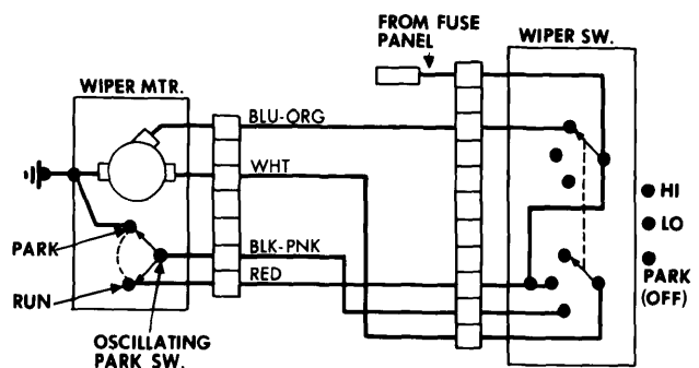
Ford Motor Co. Non-Depressed Wiper System Wiring Diagram (Exc. Intermittent Wipers) Mustang, Granada and Monarch
