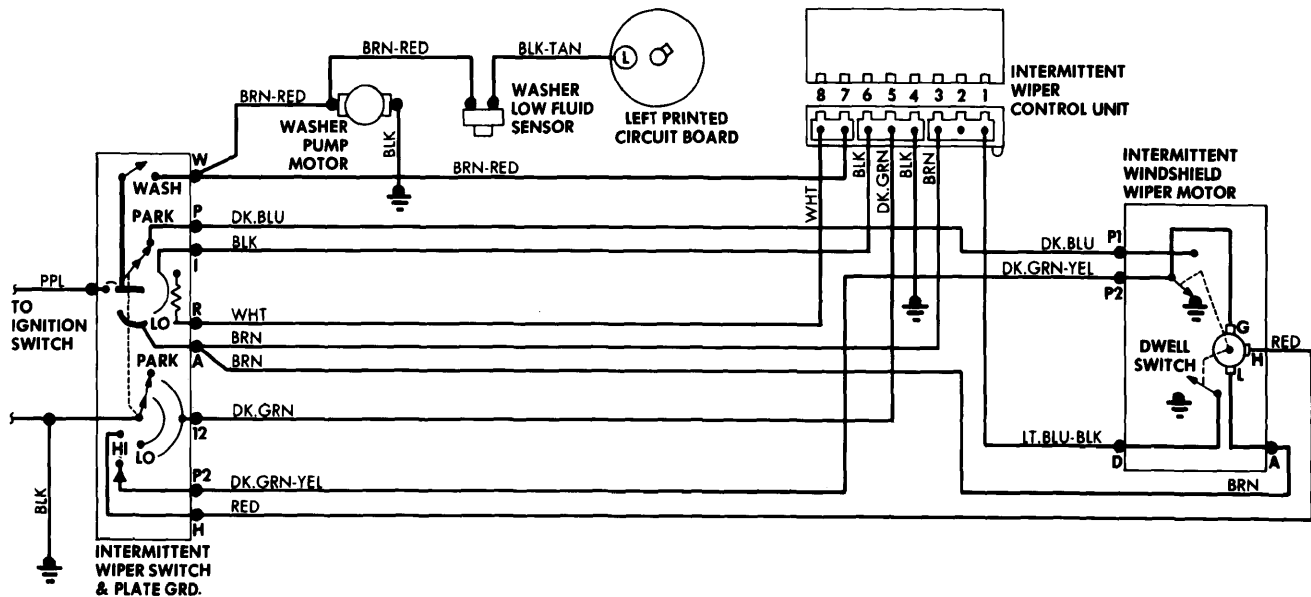
Chrysler Corp. Two-Speed Intermittent Wiper System Wiring Diagram
