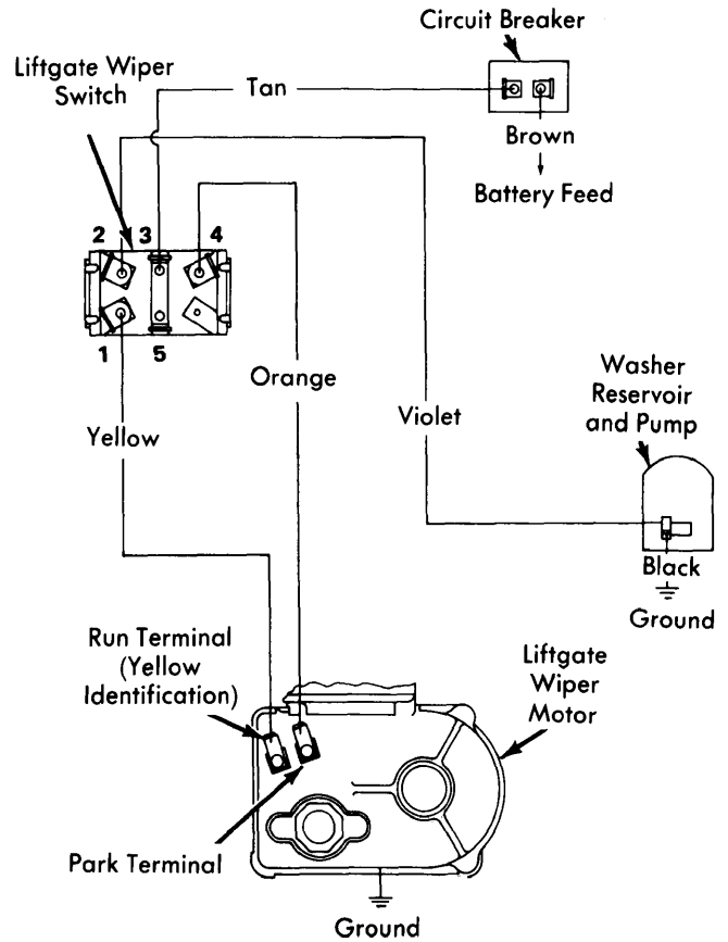
American Motors Pacer Liftgate Wiper/Washer System Wiring Diagram
