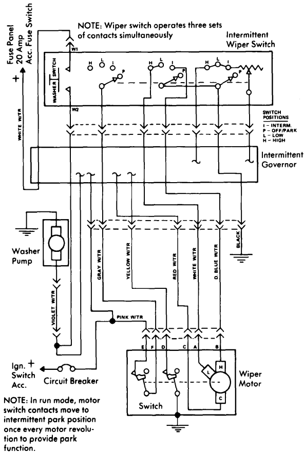
American Motors Pacer Concealed Intermittent Wiper System Wiring Diagram
