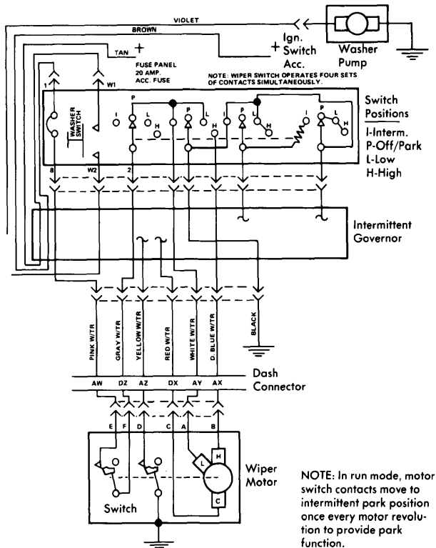
American Motors Matador Concealed Intermittent Wiper System Wiring Diagram
