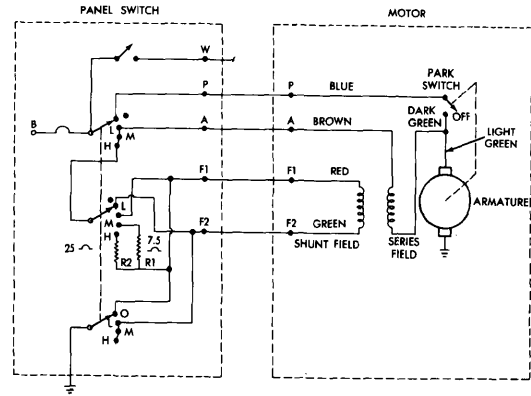
Chrysler Corp. Three-Speed Wiper System Wiring Diagram
