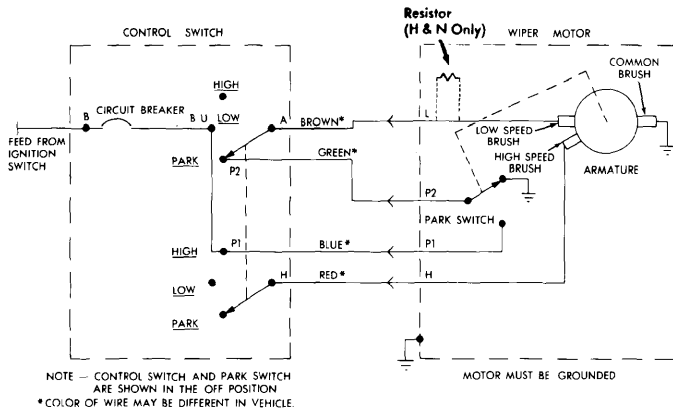
Chrysler Corp. Non-Concealed Wiper with Two-Speed Motor Wiring Diagram
