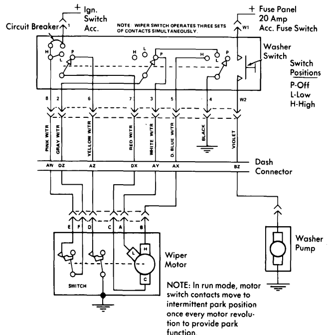
American Motors Matador Concealed Standard Windshield Wiper System Wiring Diagram
