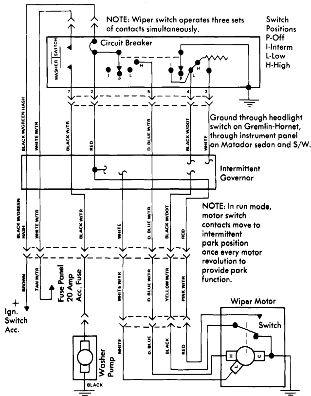
American Motors Non-Concealed Wiper System Wiring Diagram With Intermittent Governor
