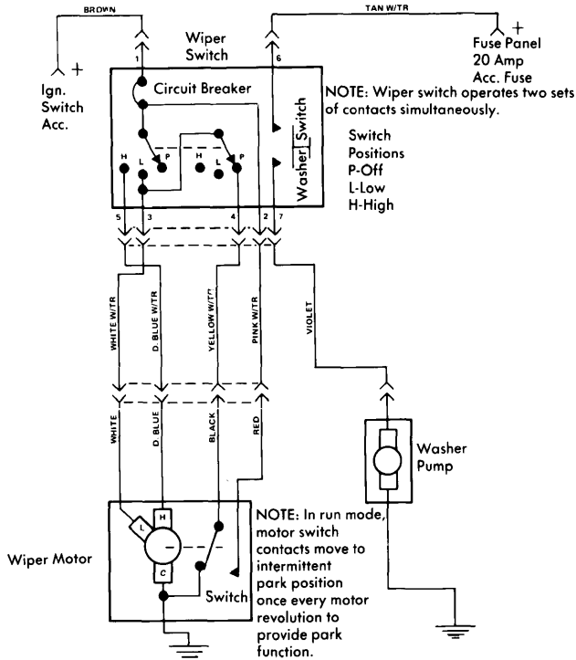
American Motors Non-Concealed Standard Wiper System Wiring Diagram
