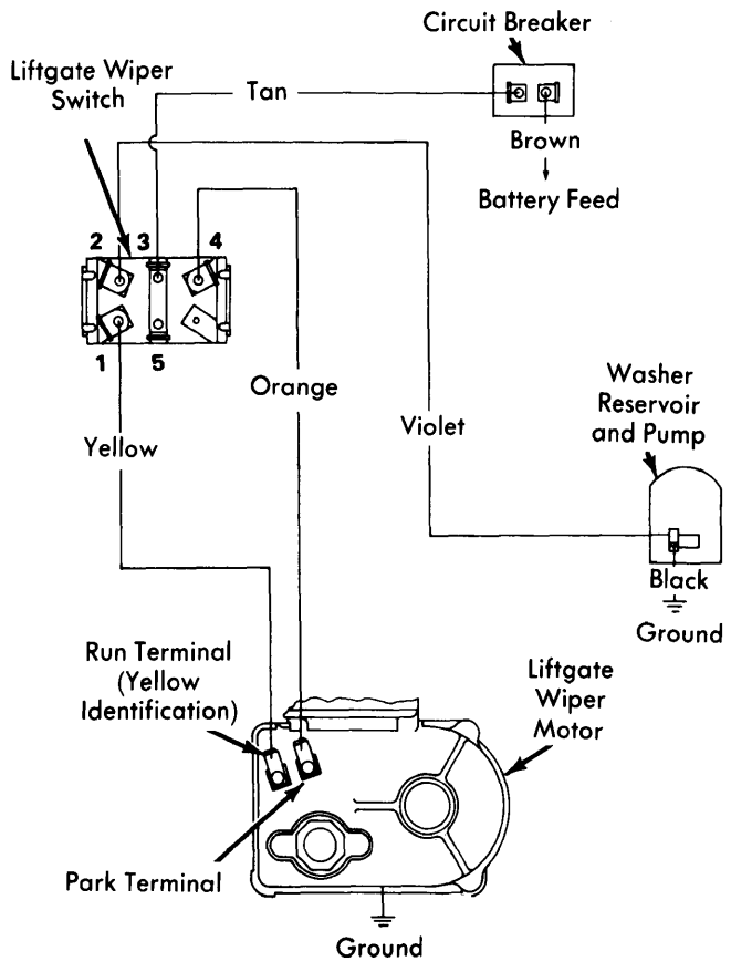
American Motors Pacer Liftgate Wiper/Washer System Wiring Diagram
