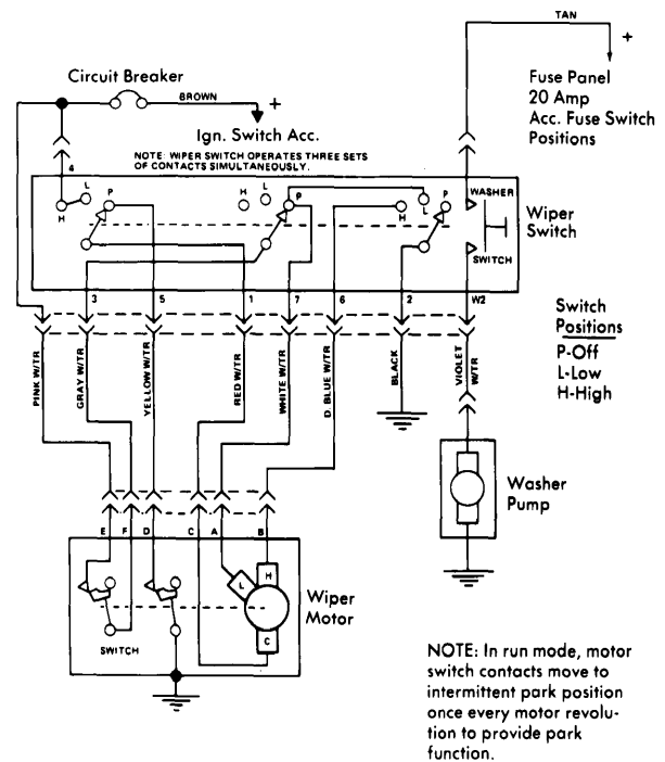
American Motors Pacer Concealed Windshield Wiper System Wiring Diagram
