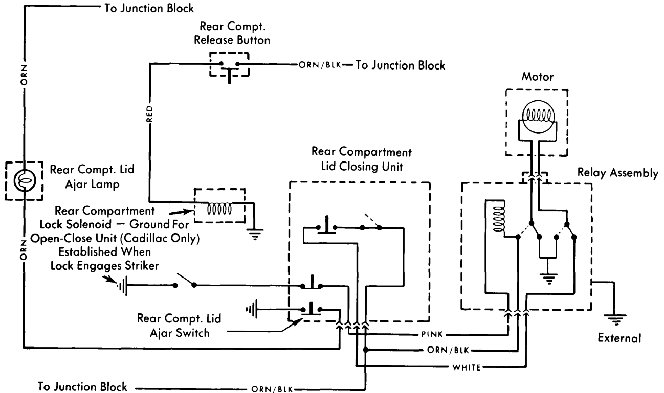
General Motors Electric Trunk Lid Latch Wiring Diagram Showing Cadillac Trunk Lid Opening and Closing Circuit
