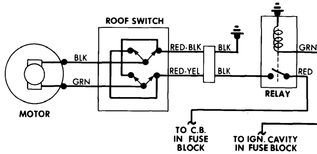
Buick Electric Sunroof Wiring Diagram Other General Motors Models Similar
