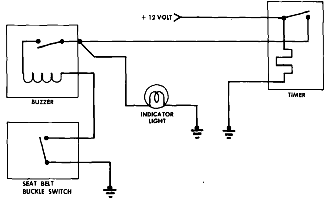
Chrysler Corp. Seat Belt Warning System Wiring Diagram
