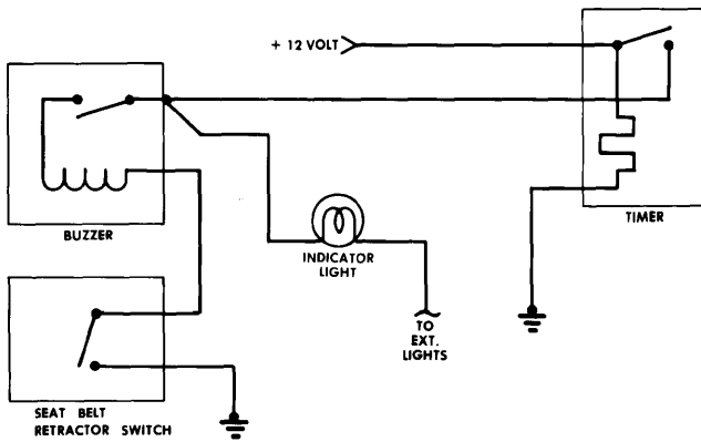
Ford Motor Co. Seat Belt Warning System Wiring Diagram
