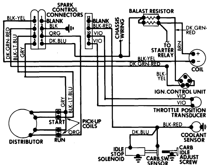
Chrysler Corp. Electronic Lean Burn System Wiring Diagram for 360", 400", and 440" Engines
