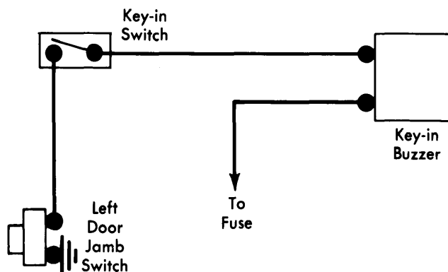
General Motors Separate Key Warning Buzzer Wiring Diagram (Buick and Chevrolet)
