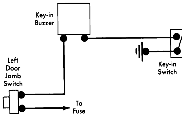
Ford Motor Co. Key Warning Buzzer Wiring Diagram
