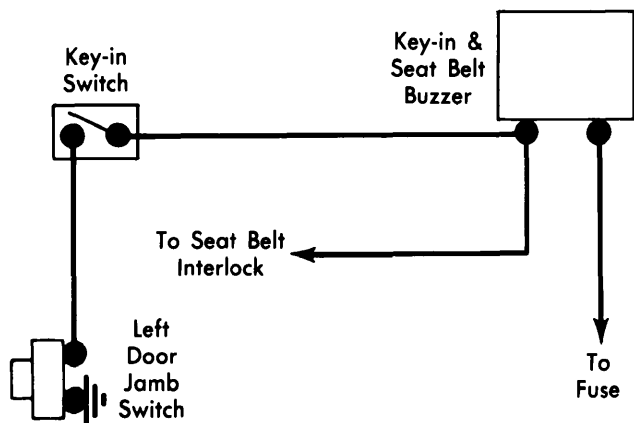
American Motors and Chrysler Corp. Key Warning Buzzer Wiring Diagram
