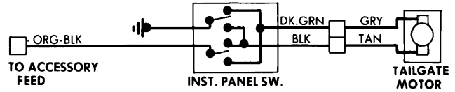
Chevrolet, Oldsmobile, & Pontiac Station Wagon Electric Tailgate Lock Wiring Diagram for Models not Equipped with Electric Door Locks
