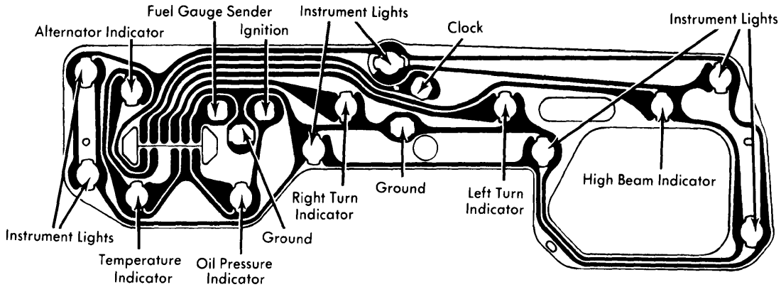
Catalina, Bonneville, and Safari Instrument Cluster with Indicator Lights
