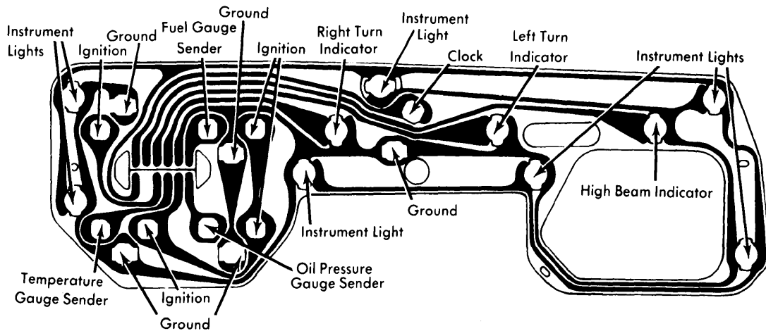
Catalina, Bonneville, and Safari Instrument Cluster with Gauges
