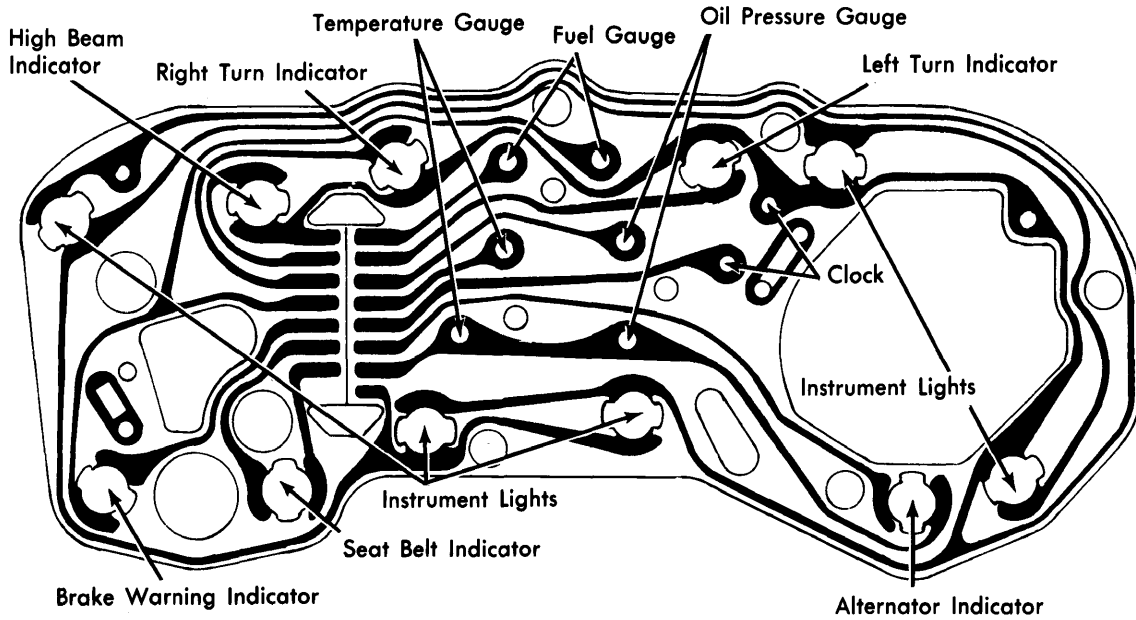
LeMans Instrument Cluster with Gauges
