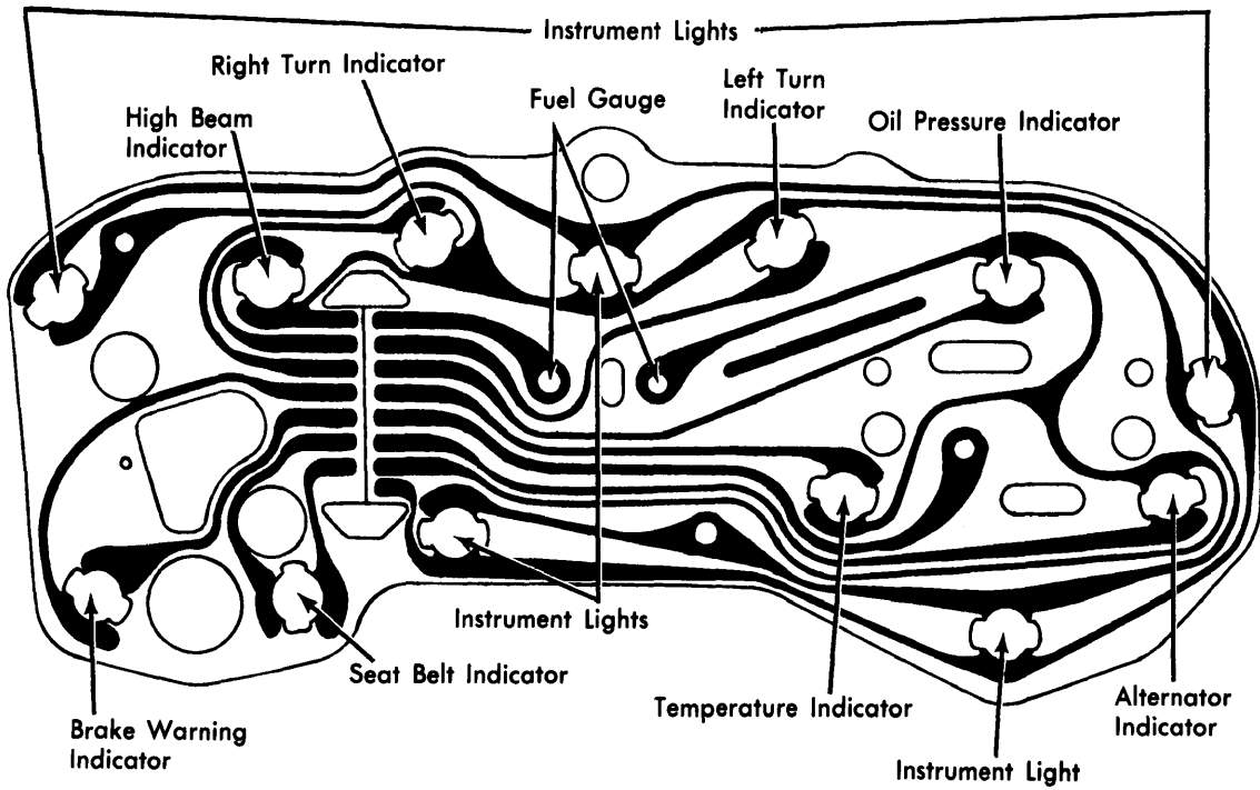
LeMans Instrument Cluster with Indicator Lights and Late Firebird Instrument Cluster with Indicator Lights
