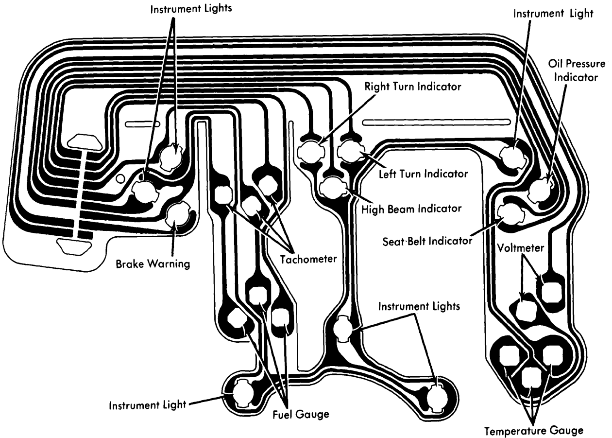
Sunbird Instrument Cluster with Gauges
