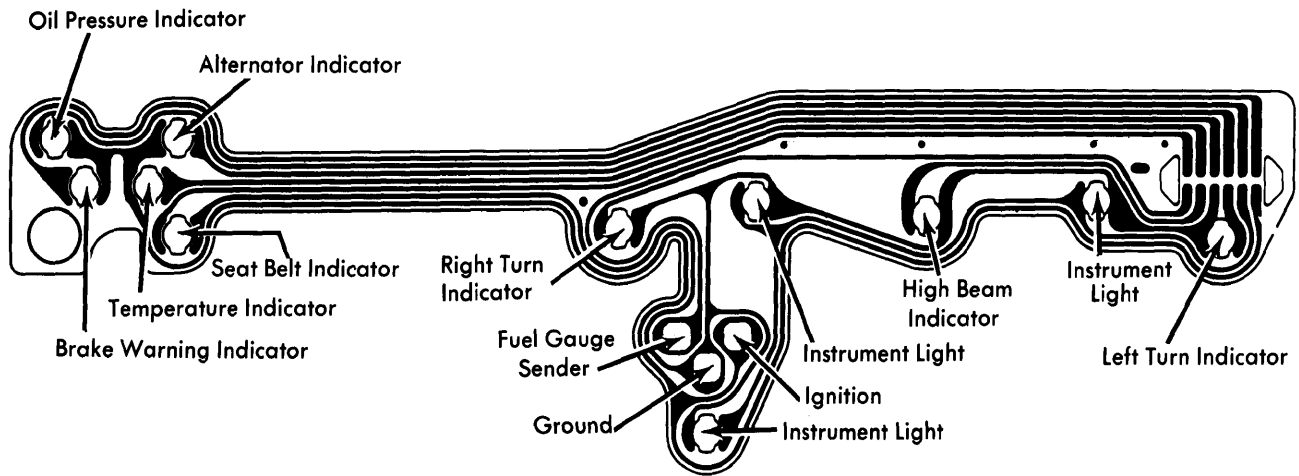
Delta 88 and NinetyEight Instrument Cluster
