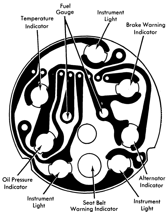
Cutlass Instrument Panel Fuel Gauge and Indicator Light Cluster without Fuel Economy Meter
