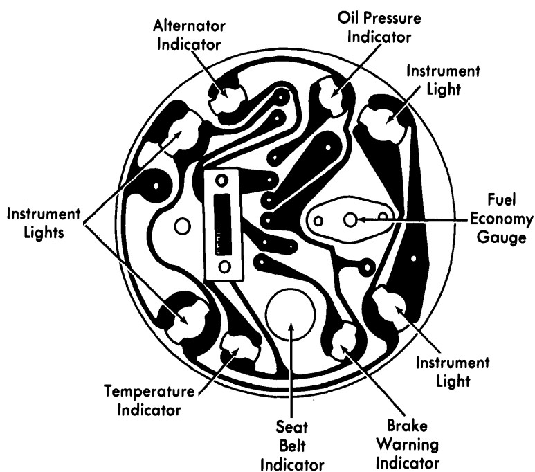
Cutlass Instrument Panel Fuel Gauge and Indicator Lights Cluster with Fuel Economy Meter
