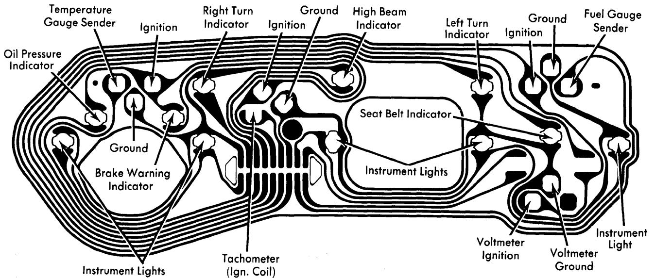
Omega Instrument Cluster with Gauges
