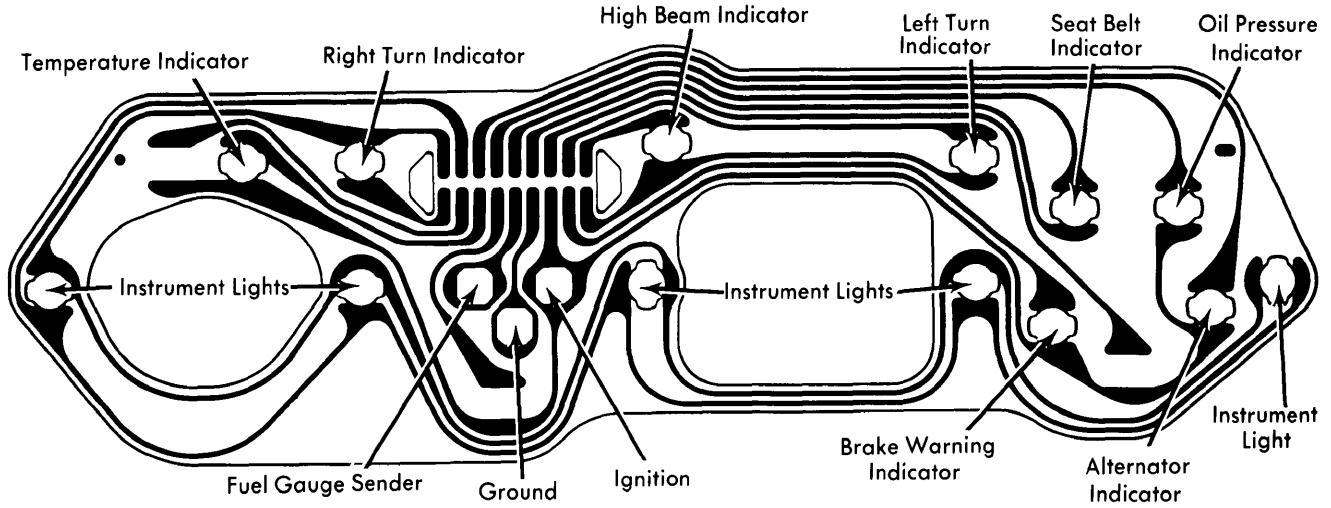
Omega Instrument Cluster with Indicator Lights
