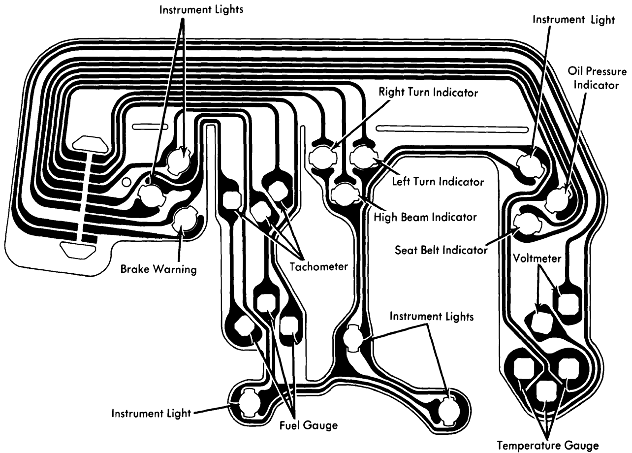
Starfire Instrument Cluster With Gauges
