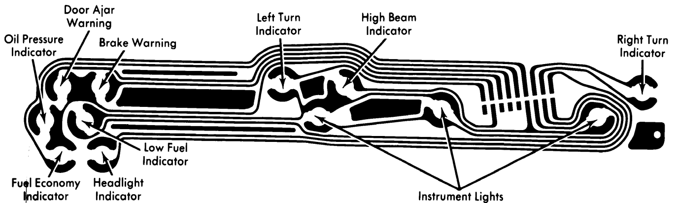
Lincoln Continental Upper (Speedometer) Instrument Cluster
