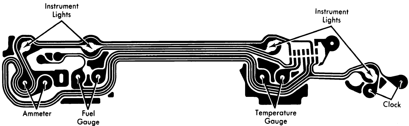
Lincoln Continental Lower Instrument Cluster
