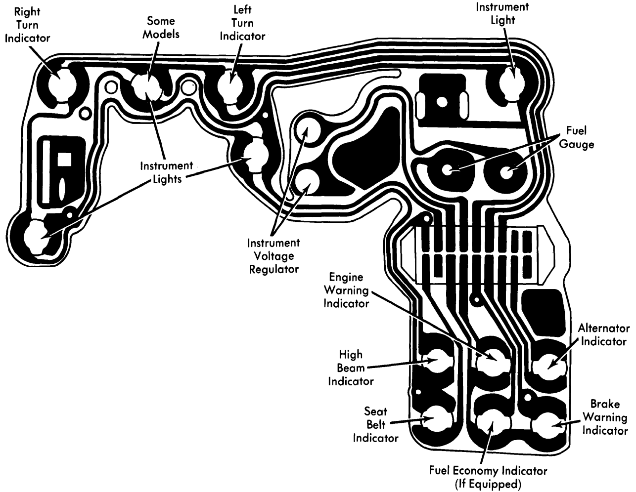
Granada and Monarch Instrument Cluster — Using Leaded Gasoline and Built After 1-2-76 and All Granada and Monarch Models Using Unleaded Gasoline
