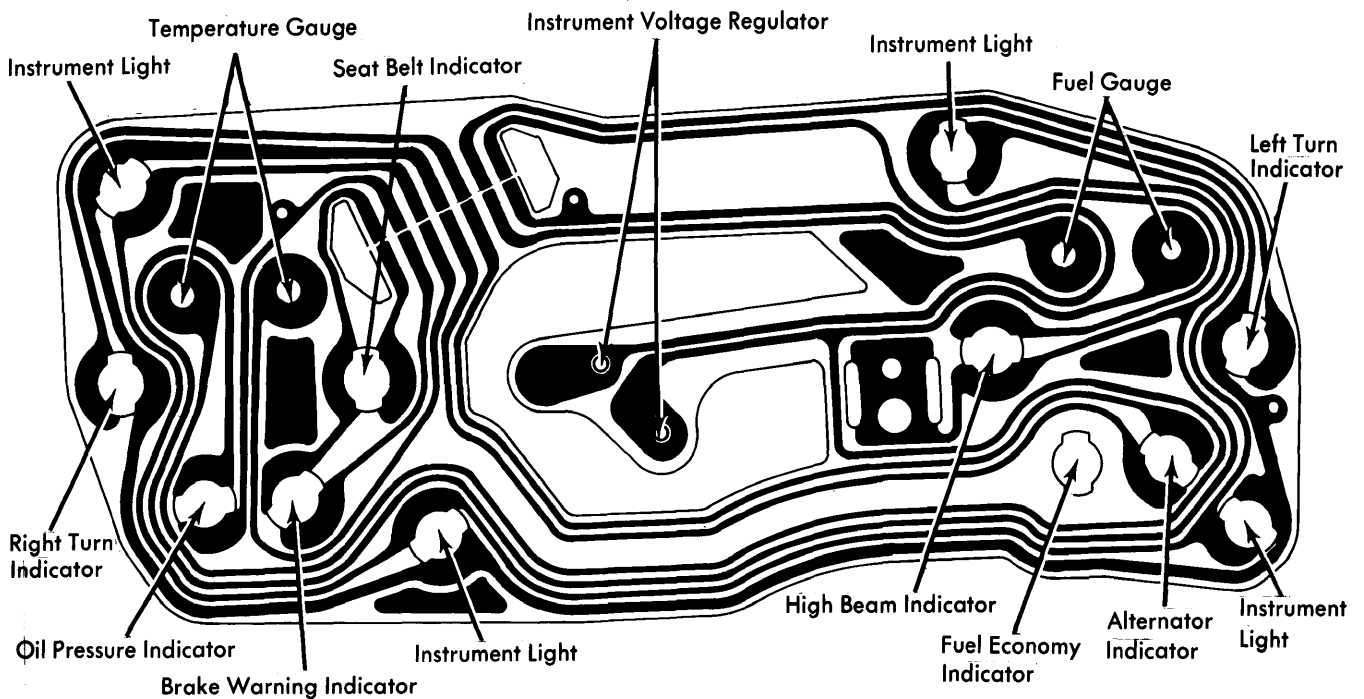
LTD II, Thunderbird, and Cougar Instrument Cluster
