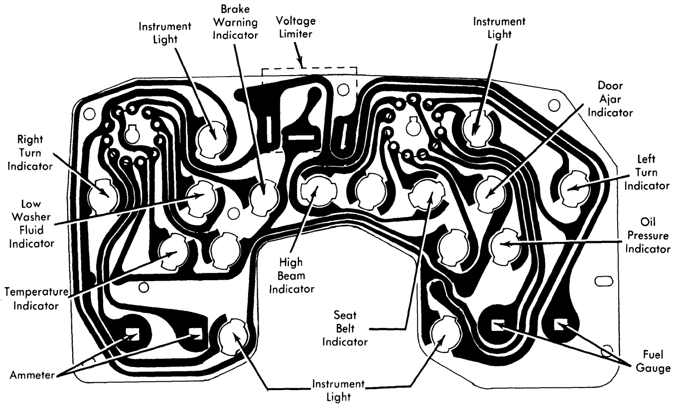
Gran Fury and Royal Monaco Instrument Cluster
