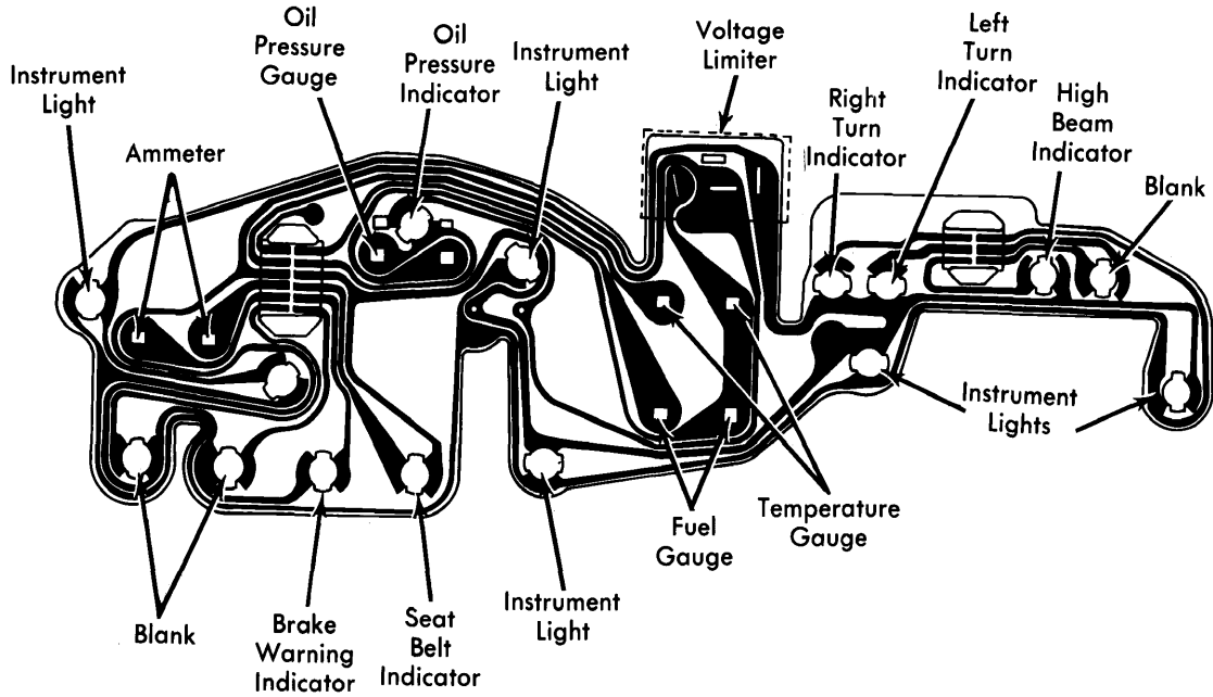
Fury, Monaco, Cordoba, and Charger Instrument Cluster without Tachometer
