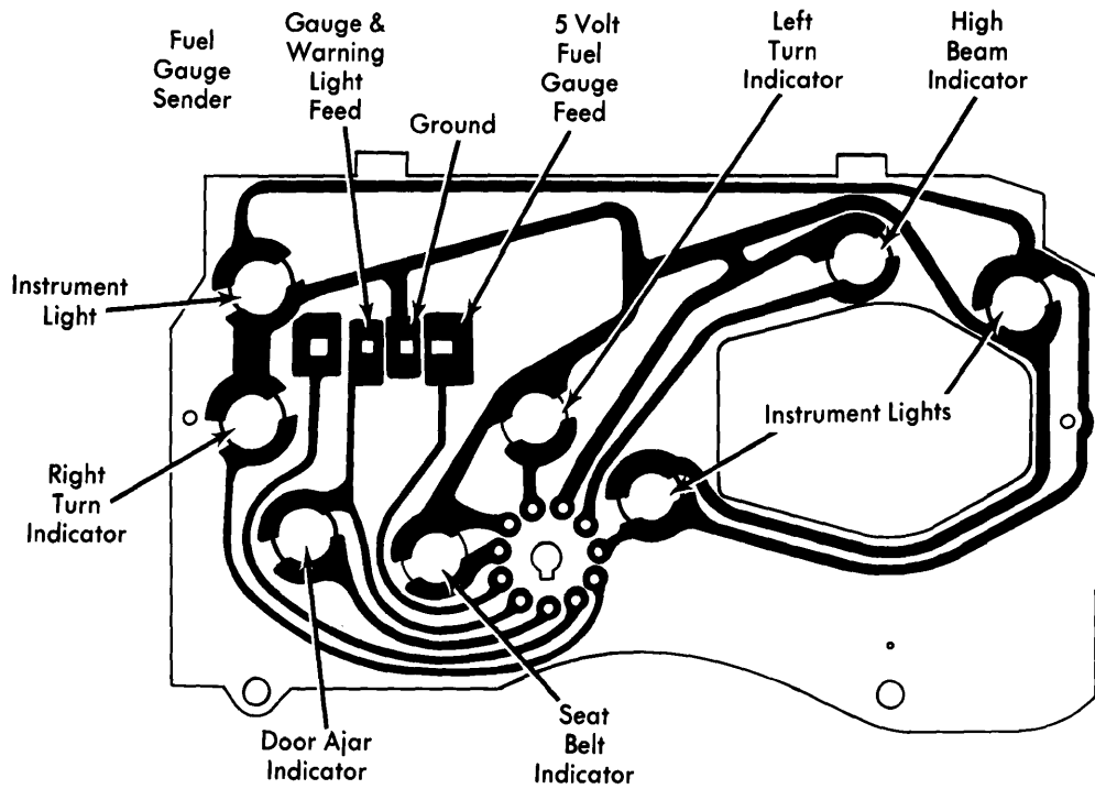
Diplomat and LeBaron Right Side Instrument Cluster
