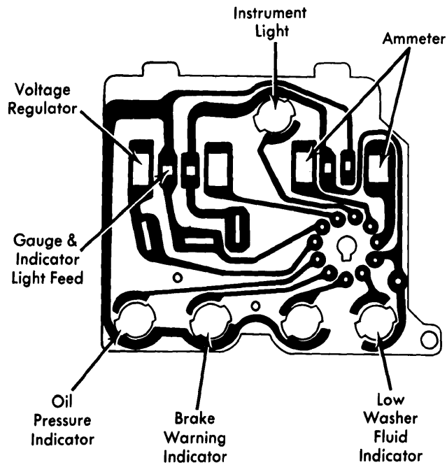
Diplomat and LeBaron Left Side Instrument Cluster
