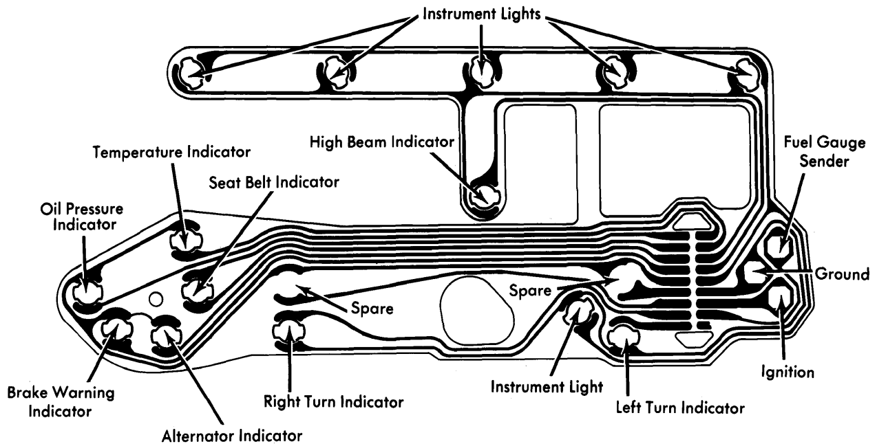
Chevrolet (including Police Vehicles) Instrument Cluster with Indicator Lights
