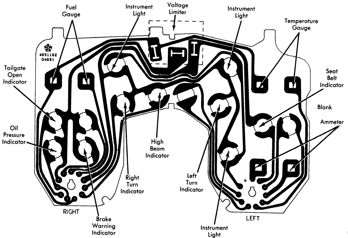
Aspen and Volare Instrument Cluster
