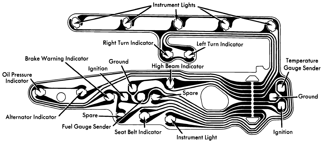
Chevrolet Instrument Cluster with Gauges
