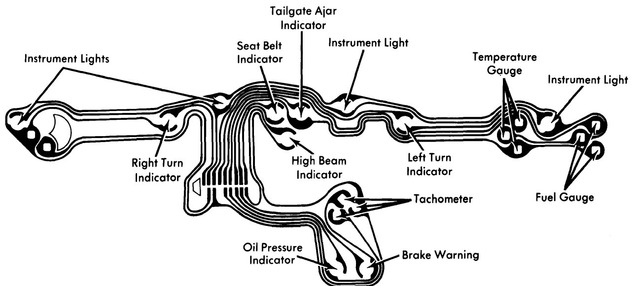
Chevelle (Super Sport) and Monte Carlo Instrument Cluster with Gauges
