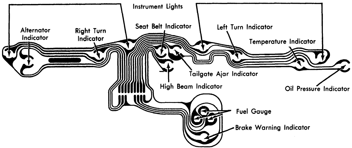
Chevelle (Super Sport) and Monte Carlo Instrument Cluster with Indicator Lights
