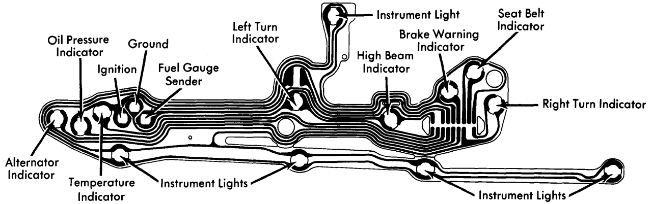
Chevelle (Standard) Instrument Cluster with Instrument Lights
