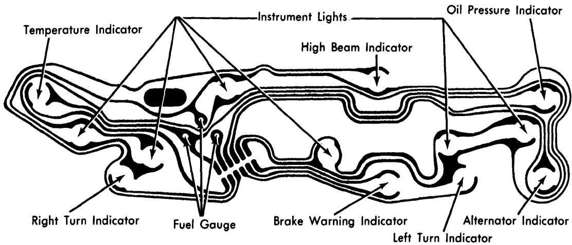
Camaro Instrument Cluster with Indicator Lights
