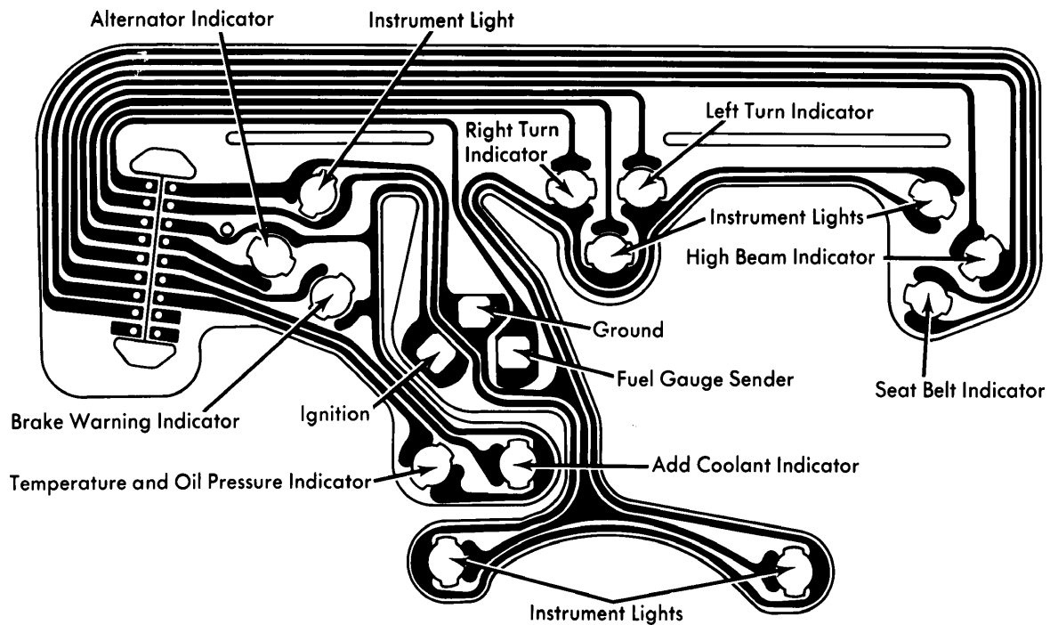
Monza and Town Coupe Instrument Cluster with Indicator Lights
