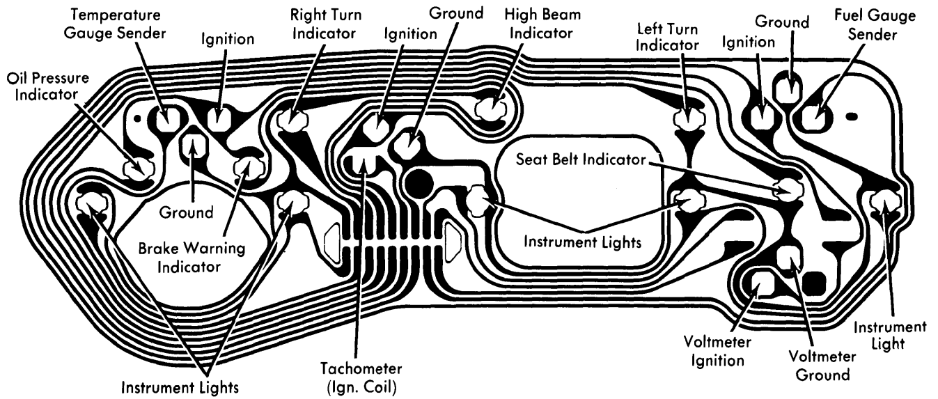
Nova Instrument Cluster with Gauges
