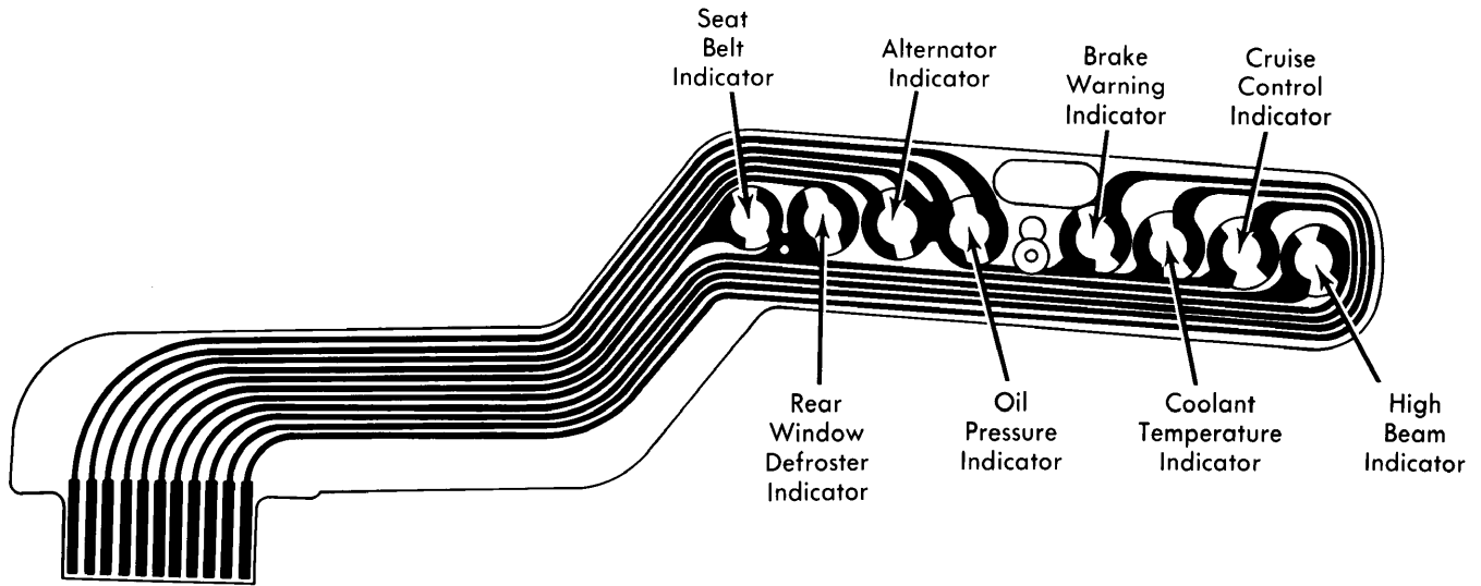
LeSabre, Estate Wagon, Electra, and Riviera High-Level Indicator Lights Cluster
