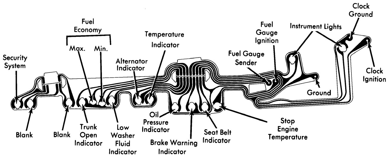
Cadillac (except Seville and Eldorado) High-Level Indicator Lights and Fuel Gauge Cluster
