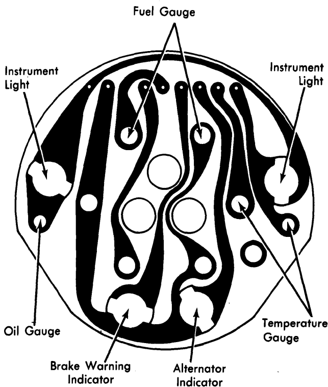
Century and Regal Instrument Cluster with Gauges
