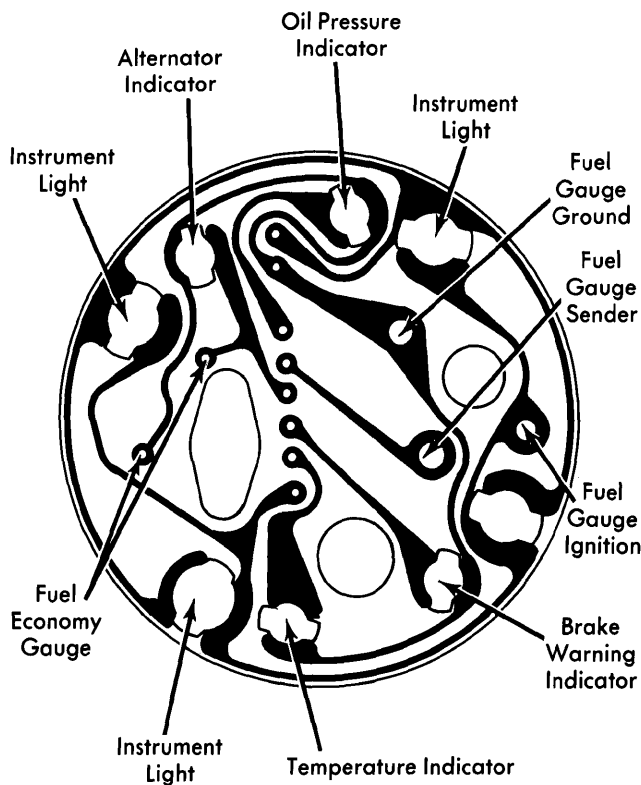
Century and Regal Instrument Cluster with Indicator Lights and Fuel Economy Gauge
