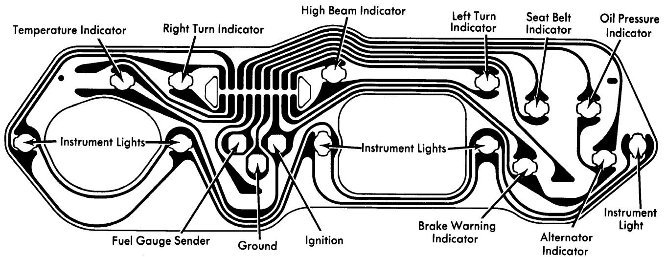
Skylark Instrument Cluster with Indicator Lights
