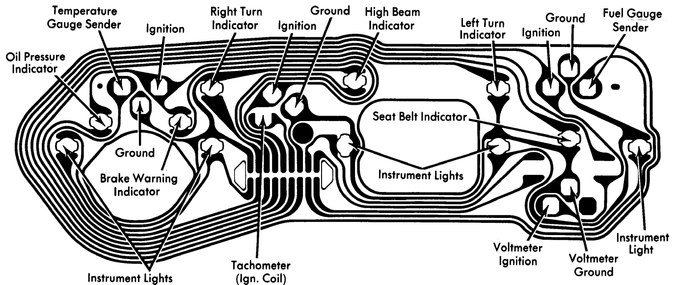
Skylark Instrument Cluster with Gauges
