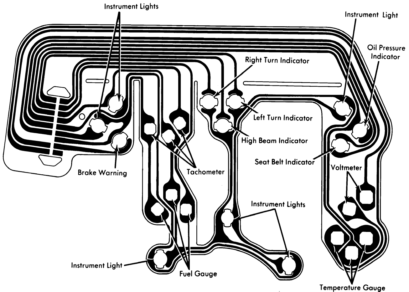
Skyhawk Instrument Cluster with Gauges
