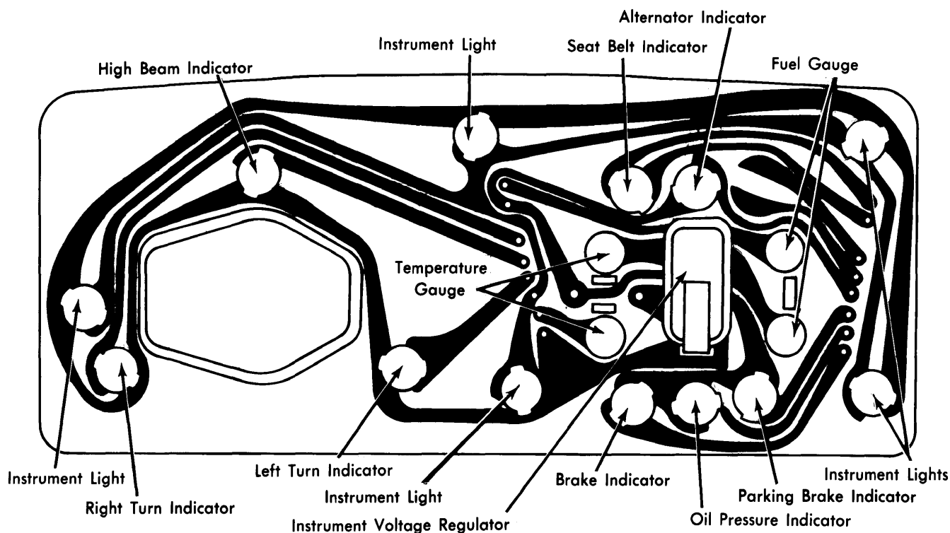
Matador Instrument Cluster with Fuel Economy Gauge in Clock Opening
