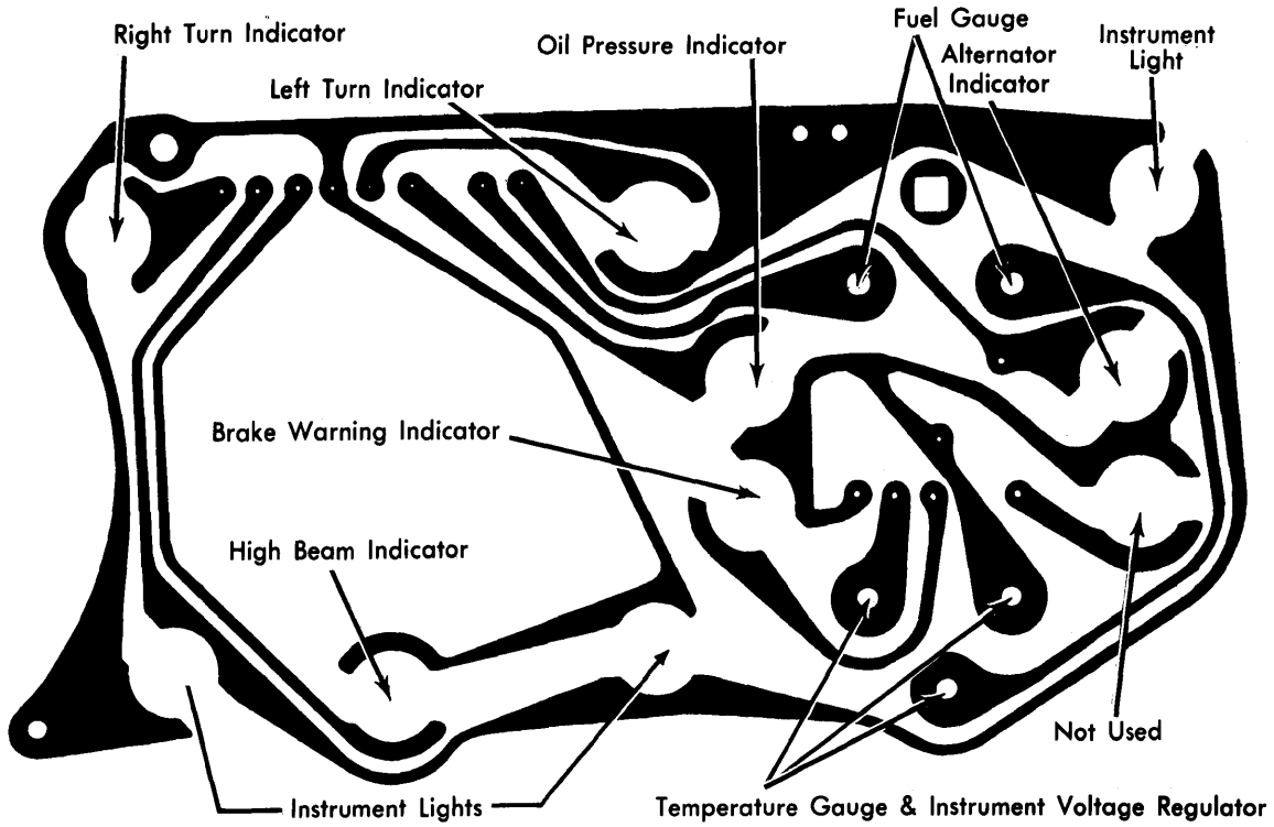
Hornet Instrument Cluster with Clock and Gremlin Instrument Cluster with Rally Gauges and Fuel Economy Gauge
