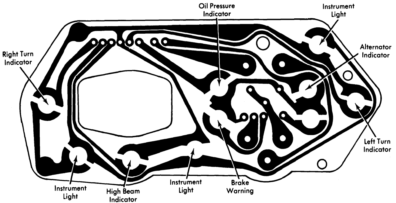
Gremlin Instrument Cluster without Rally Gauges
