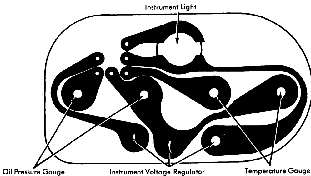
International Harvester Scout II, Traveler and Terra Temperature and Oil Pressure Gauge Circuit
