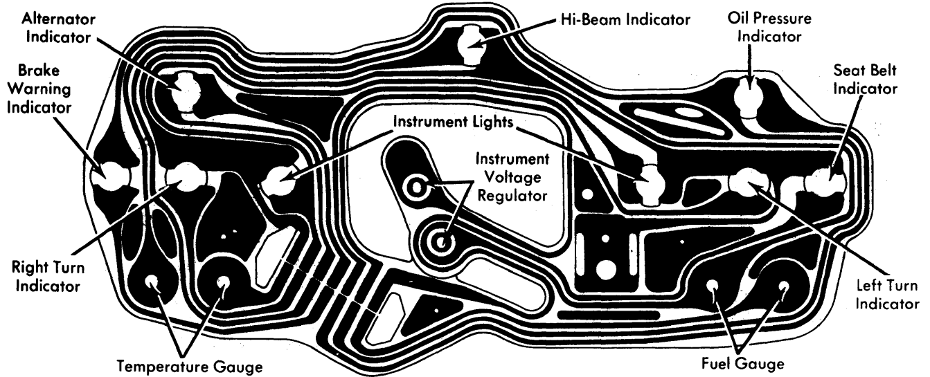
Ford "E" and "F" (All Models) With Alternator and Oil Pressure Indicator Lights
