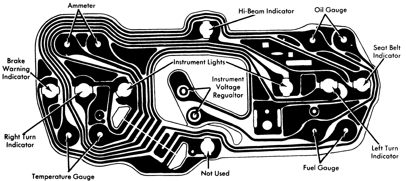
Ford "E" and "F" (All Models) With Ammeter and Oil Gauge
