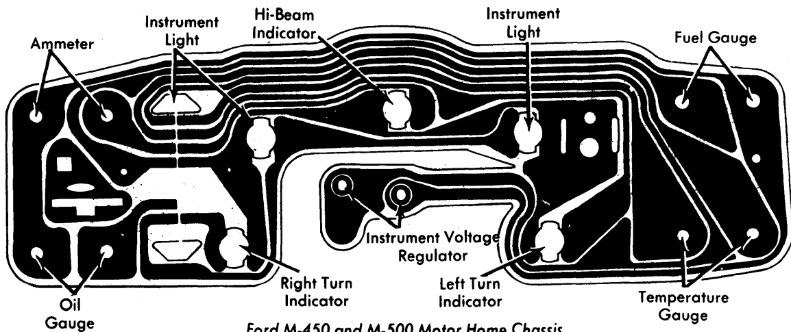
Ford M-450 and M-500 Motor Home Chassis
