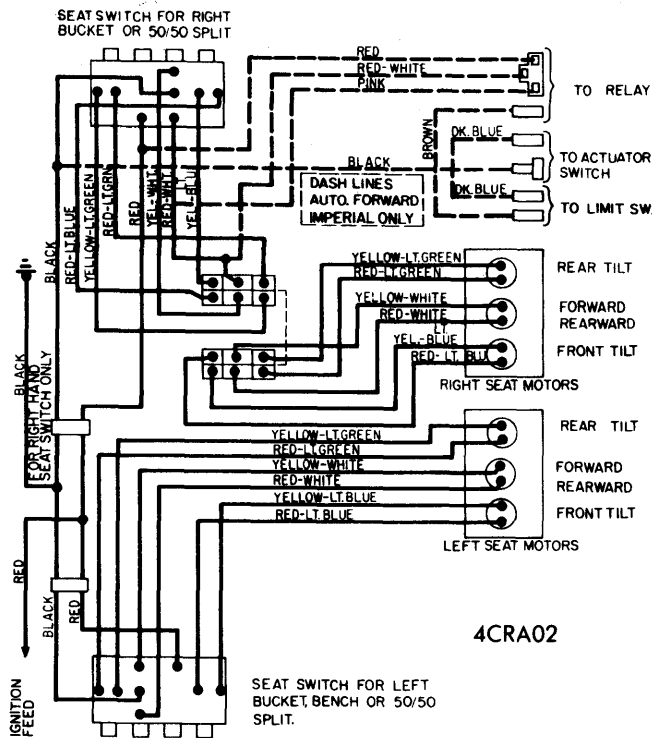
CHRYSLER CORP. POWER SEAT WIRING
