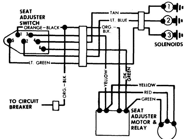
GENERAL MOTORS 4-WAY & 6-WAY POWER SEAT WIRING
