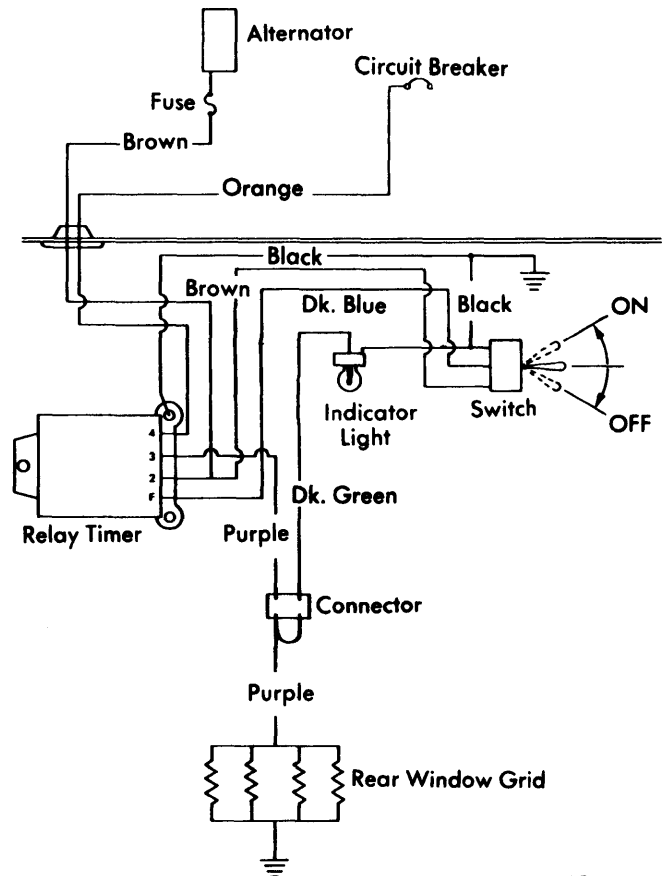
HEATED REAR WINDOW SCHEMATIC ("H" BODY)
