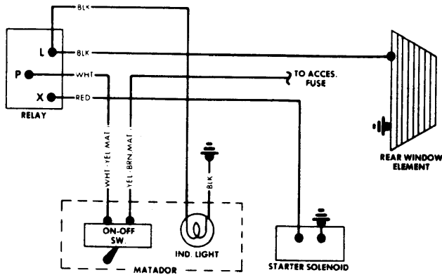
AMERICAN MOTORS HEATED REAR WINDOW WIRING
