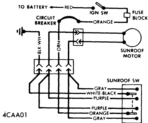
CADILLAC SUNROOF WIRING
