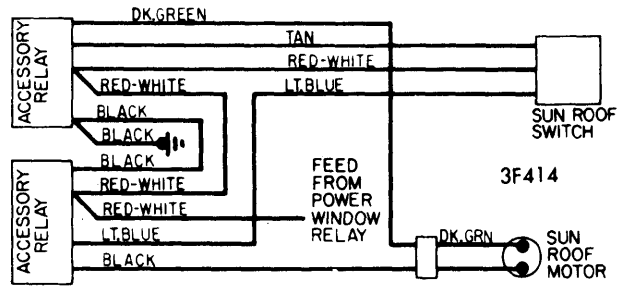
BUICK SUNROOF WIRING
