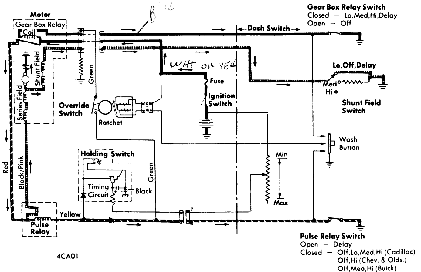
GENERAL MOTORS MODIFIED PULSE WIPER WIRING (CADILLAC - "LO" SPEED SHOWN)
