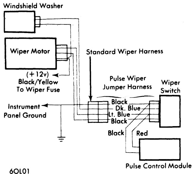
GENERAL MOTORS PULSE CONTROL WIPER SYSTEM WIRING
