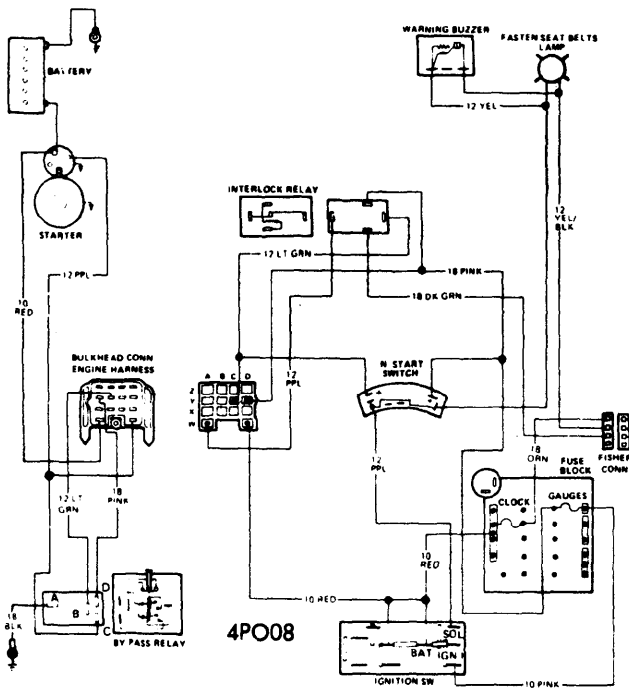
PONTIAC SEAT BELT STARTER INTERLOCK WIRING, AUTOMATIC TRANSMISSION (EXC. FIREBIRD)
