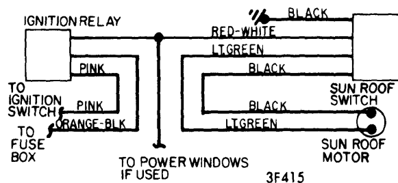
CENTURY, REGAL, CHEVELLE, MONTE CARLO, CUTLASS LE MANS, GRAND PRIX & GRAND AM SUNROOF WIRING DIAGRAM
