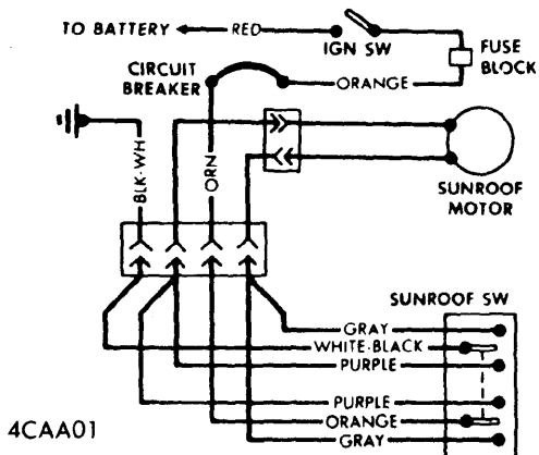
CADILLAC SUNROOF WIRING
