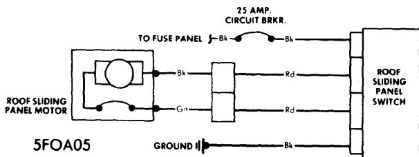
FORD MOTOR CO. SUNROOF WIRING DIAGRAM
