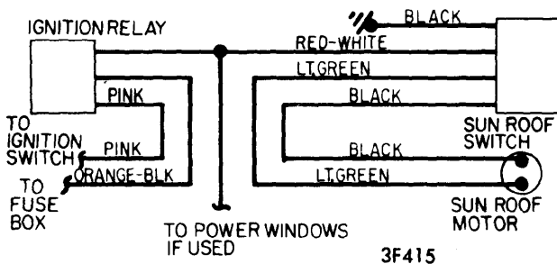
CHEVELLE, MONTE CARLO, LE MANS, GRAND PRIX CUTLASS, CENTURY & REGAL SUNROOF WIRING
