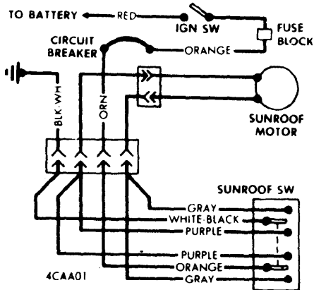
CADILLAC SUNROOF WIRING DIAGRAM
