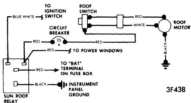
CHRYSLER SUNROOF WIRING
