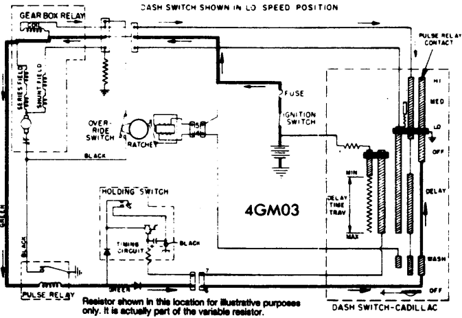
PULSE WIPER WIRING DIAGRAM (CADILLAC)
