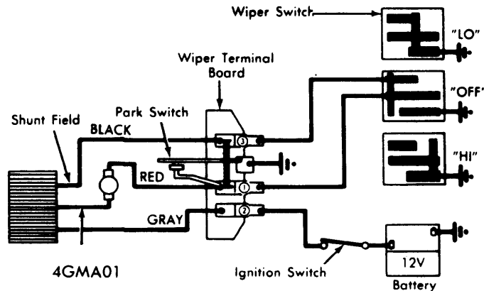
GENERAL MOTORS SQUARE-MOTOR
