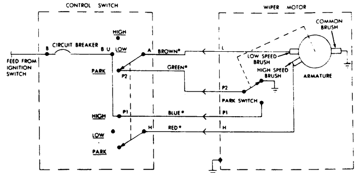
CHRYSLER CORP. 2-SPEED MOTOR WIRING (NON-CONCEALED WIPERS) 5CH02
