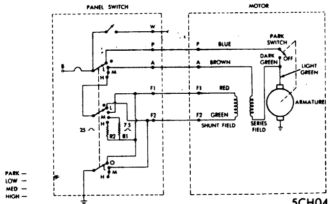
CHRYSLER CORP. 3-SPEED MOTOR WIRING 5CH04
