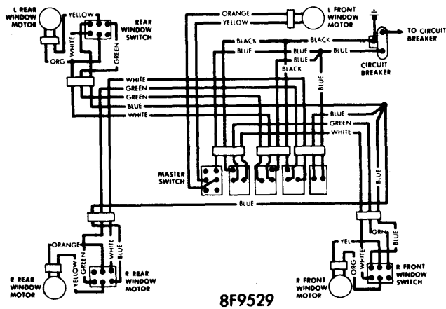
AMERICAN MOTORS POWER WINDOW WIRING
