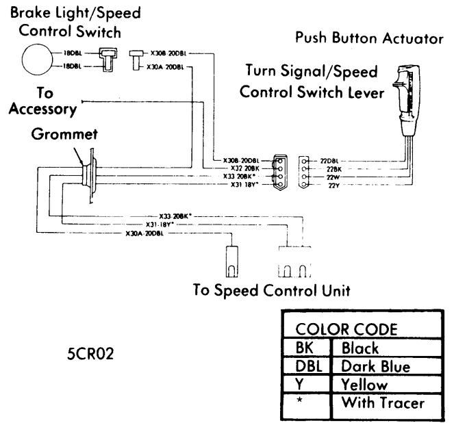
CHRYSLER CORP. SPEED CONTROL
