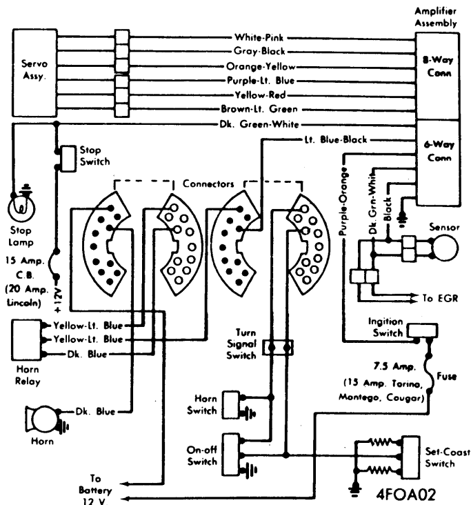
FORD MOTOR CO. SPEED CONTROL WIRING
