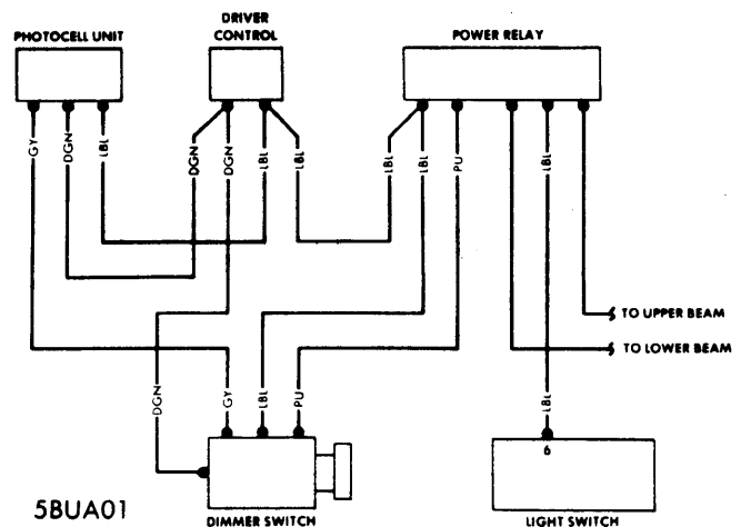
GENERAL MOTORS TWILIGHT SENTINEL
