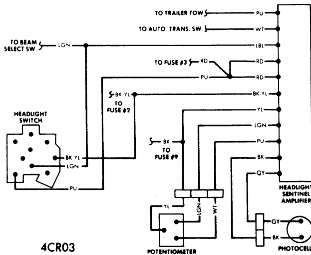
CHRYSLER CORP. SAFE GUARD SENTINEL
