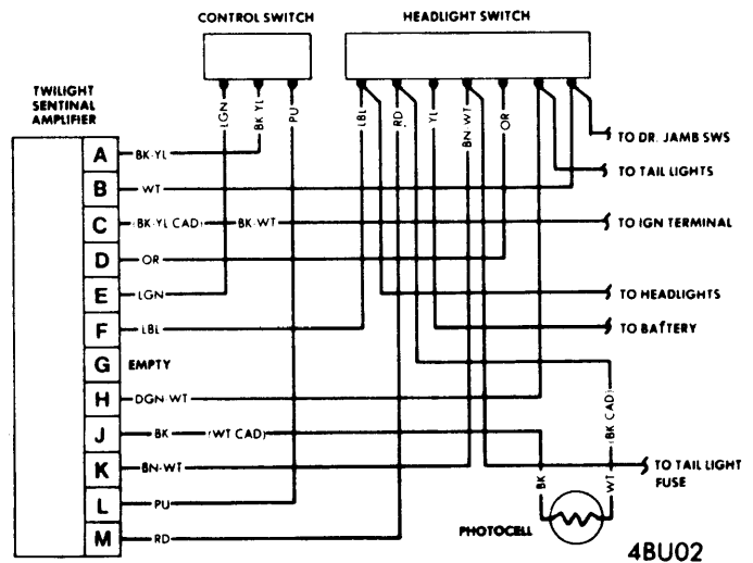
GENERAL MOTORS TWILIGHT SENTINEL
