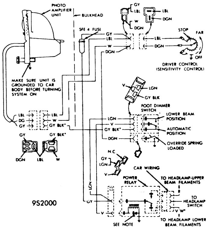
CHRYSLER CORP. AUTOMATIC BEAM CHANGER
