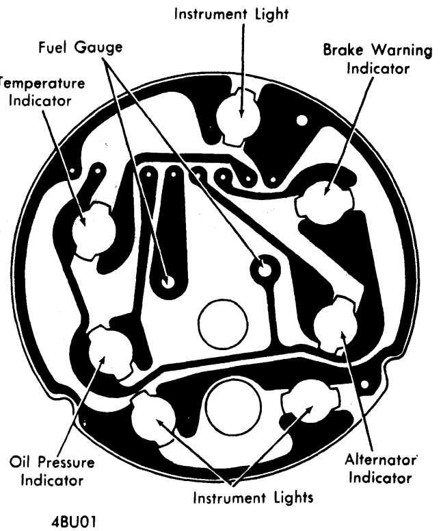
BUICK CENTURY & REGAL (WITH INDICATOR LIGHTS)
