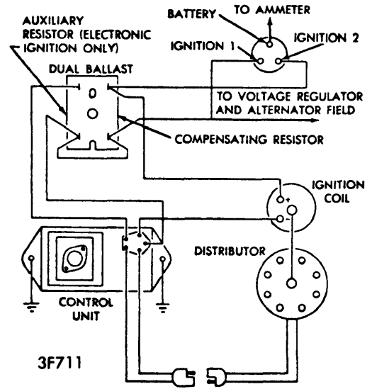
CHRYSLER CORP. ELECTRONIC IGNITION SYSTEM WIRING
