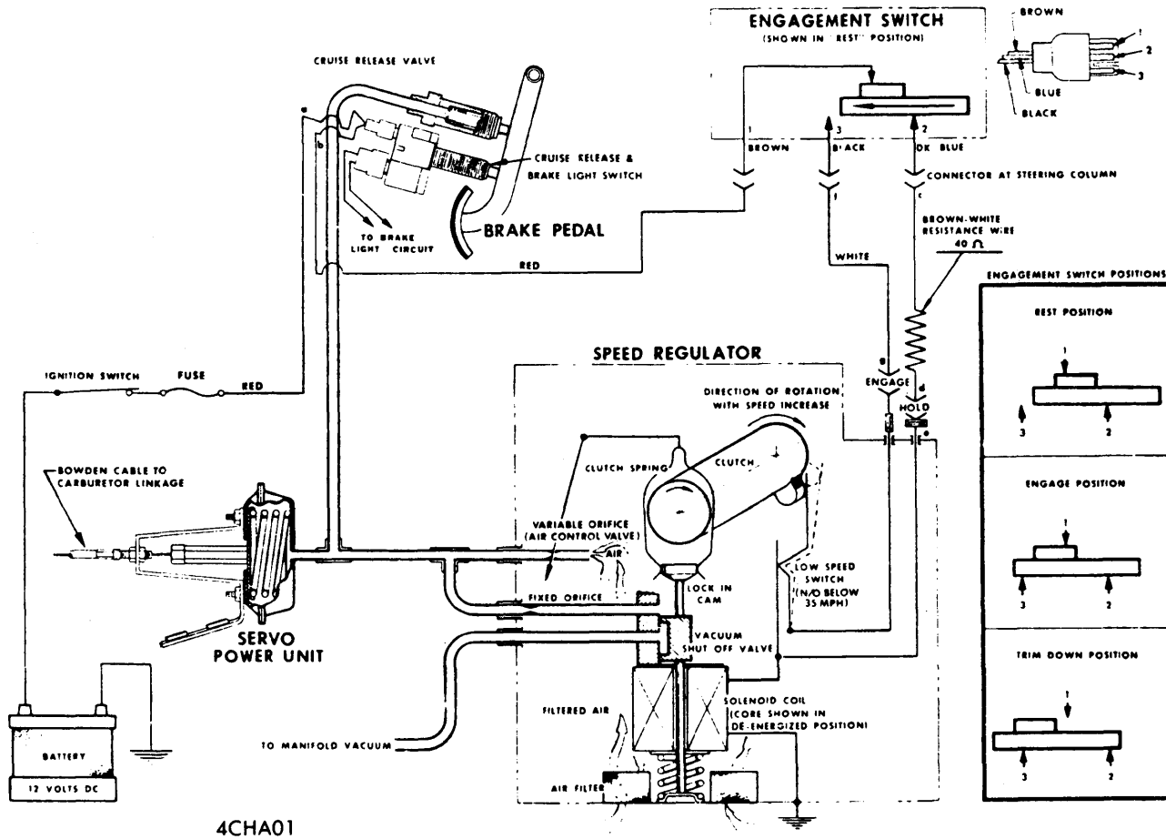
CHEVROLET CRUISE MASTER WIRING
